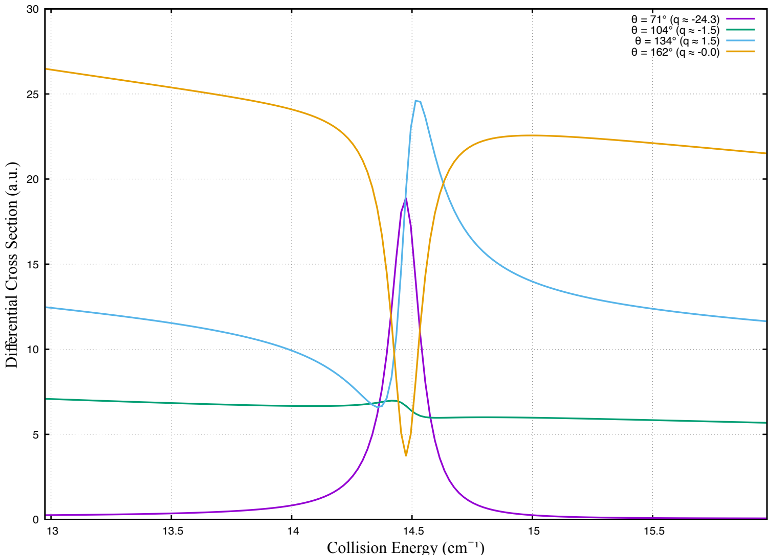
H+Xe: Archetypal Fano Resonance Profiles ( l=6 , E_r=14.475\text{ cm}^{-1} )
