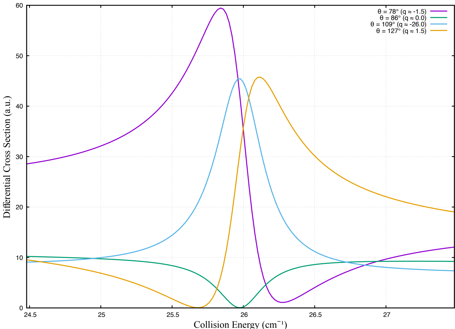
H+Xe: Archetypal Fano Resonance Profiles ( l=7 , E_r=25.98 \text{ cm}^{-1} )
