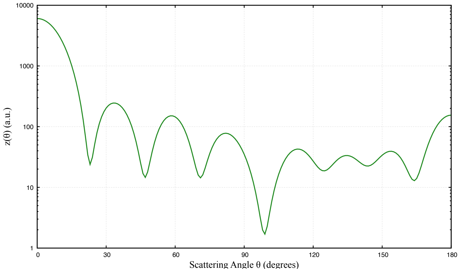
H+Xe: Background Factor z(\theta) ( l=8 )
