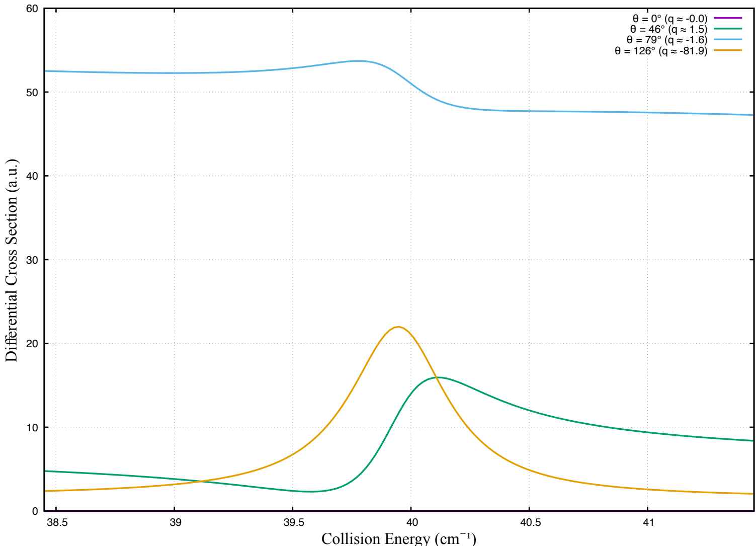
H+Xe: Archetypal Fano Resonance Profiles ( l=8 , E_r=39.95 \text{ cm}^{-1} )
