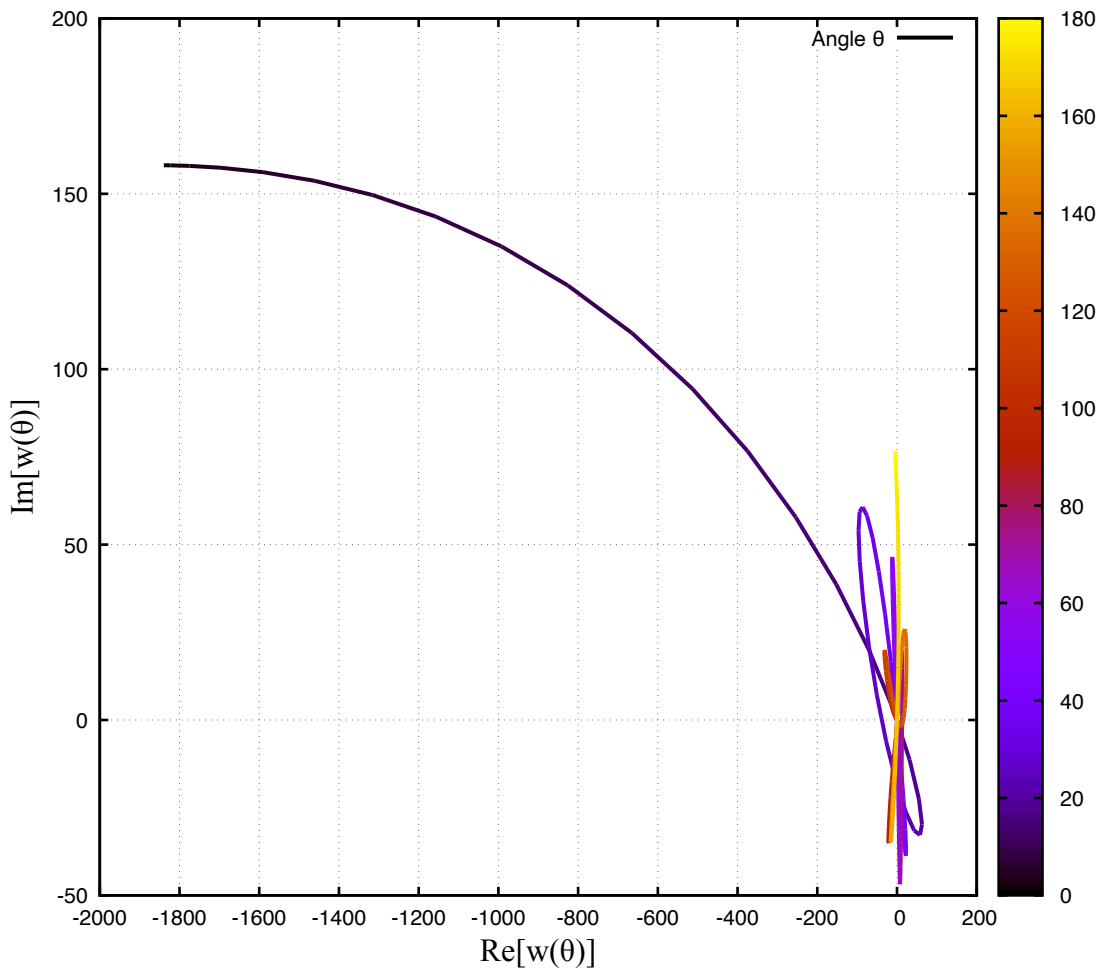
H+Xe: Complex w(\theta) Trajectory ( l=8 )
