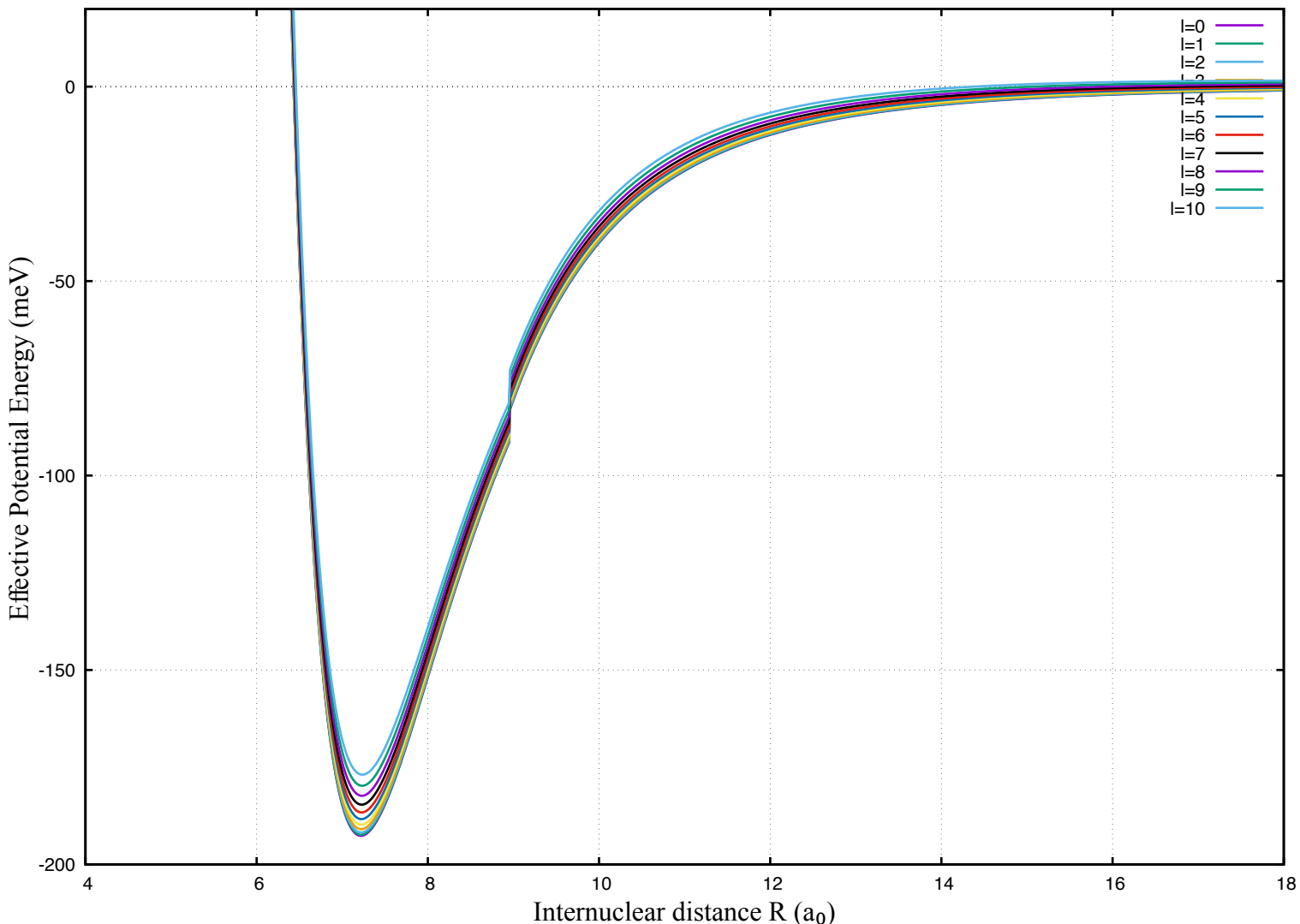
H+Xe: Effective Interaction Potentials
