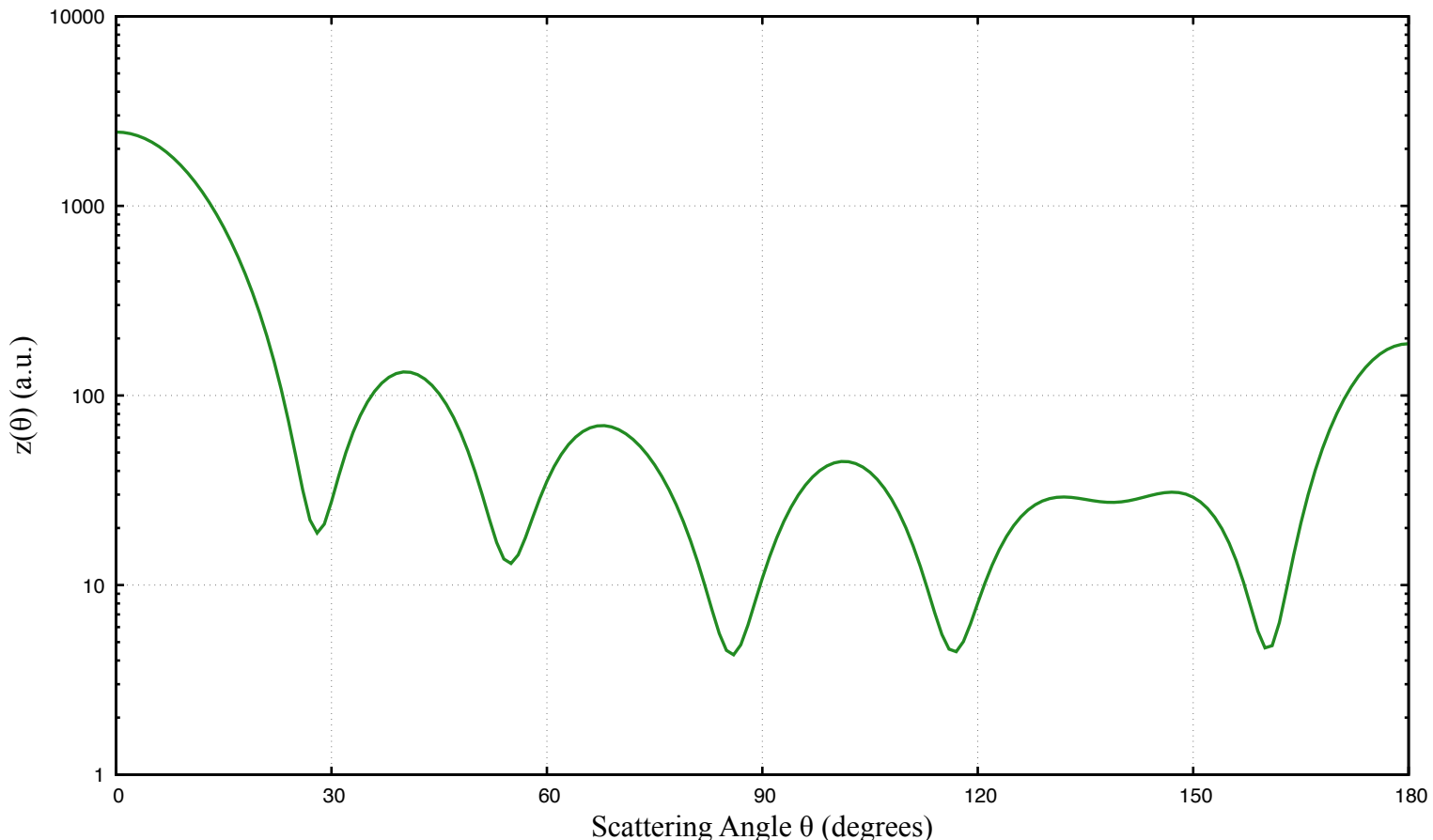
H+Xe: Background Factor z(\theta) ( l=7 )
