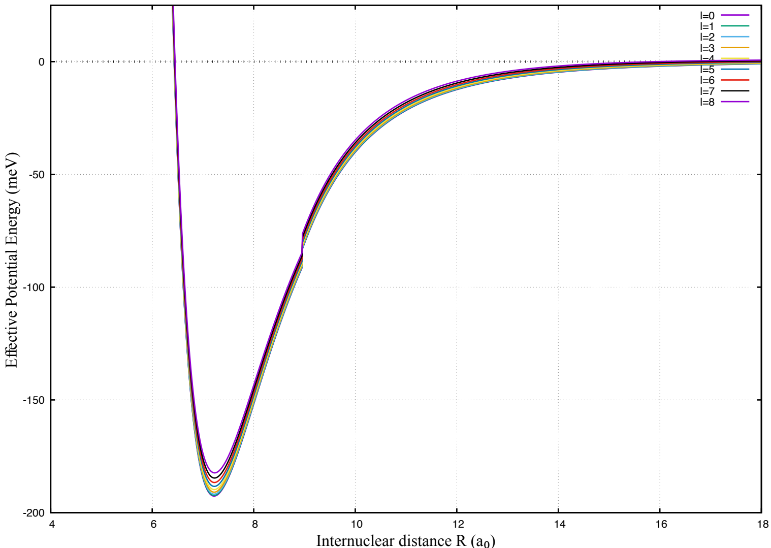
H+Xe: Effective Interaction Potentials ( l=0 to 8)
