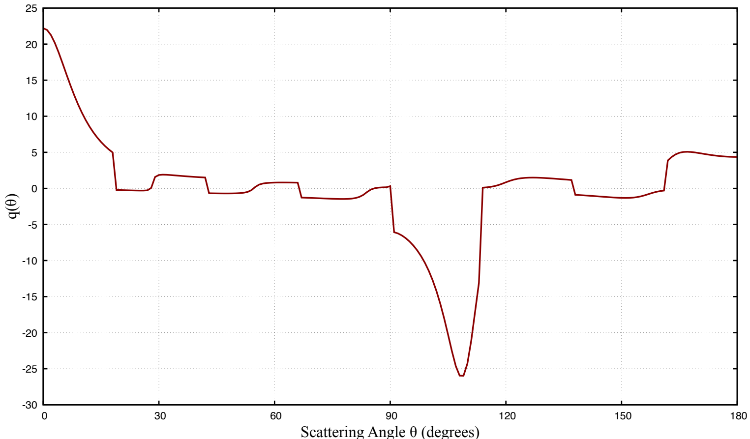
H+Xe: Angle-Dependent Fano q-parameter ( l=7 )
