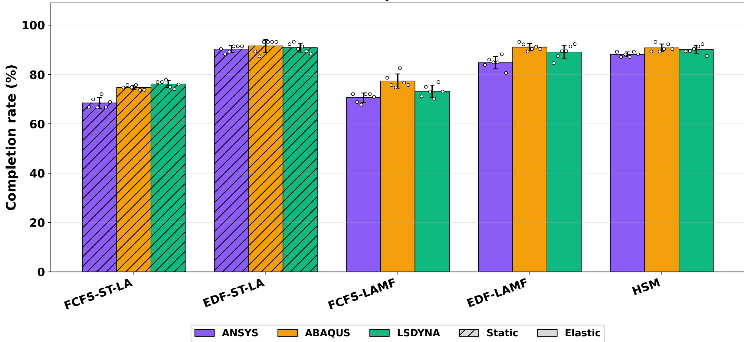
Per-solver completion at N = 300
