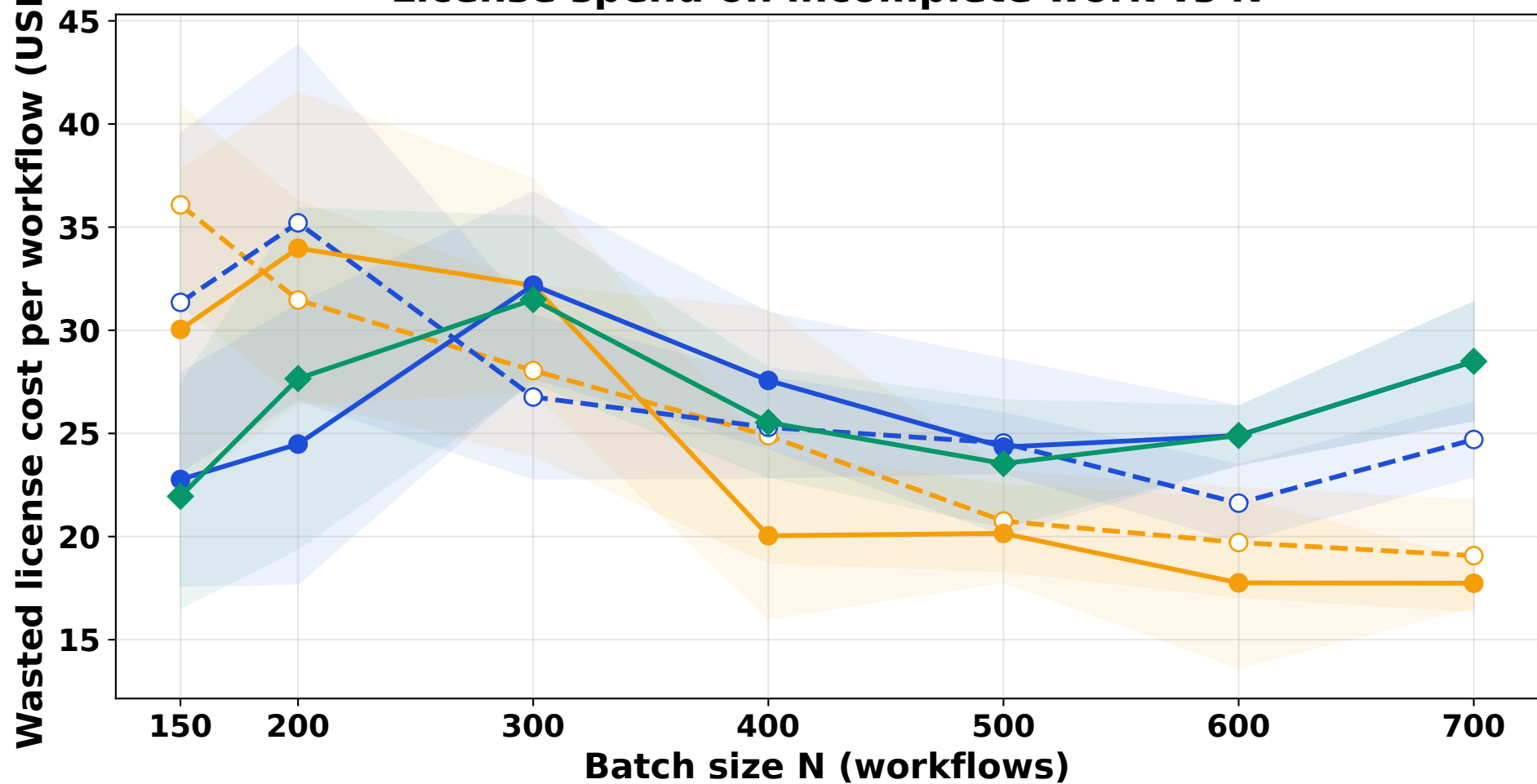
License spend on incomplete work vs N
