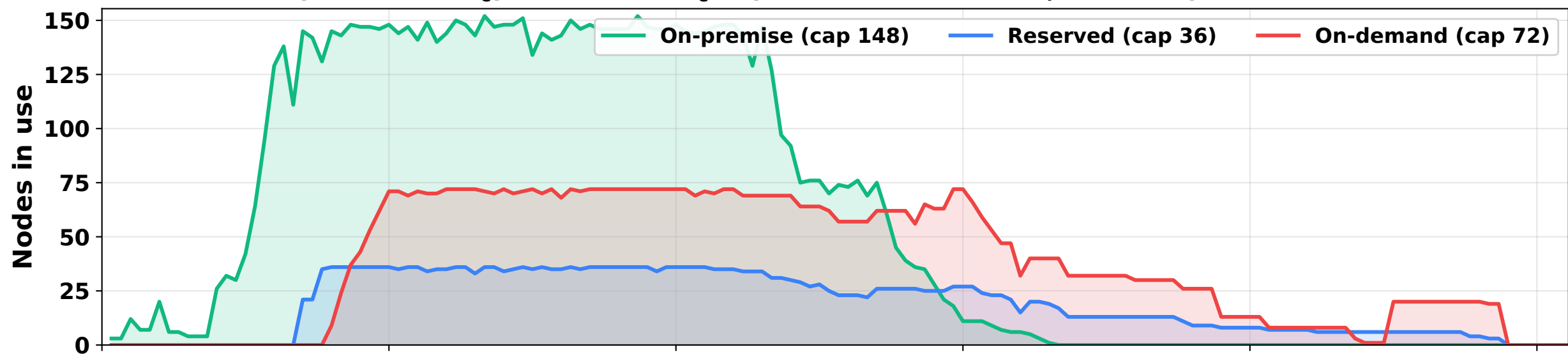
Lowest-miss (EDF-ST c ): EDF-ST c (on-demand cost: 4,608 USD)
