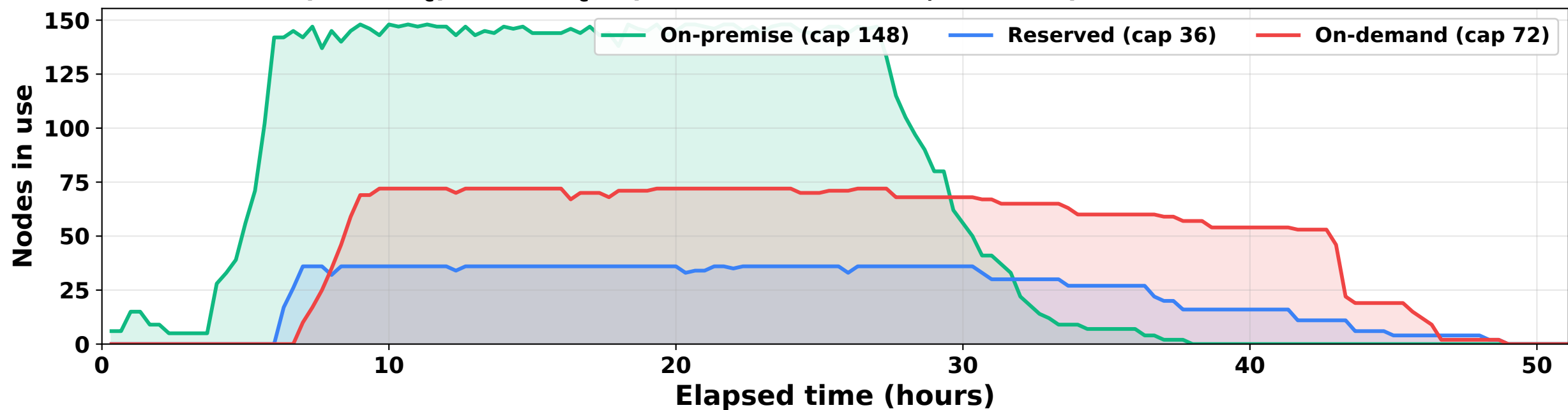
Lowest-miss (EDF-ST c ): EDF-ST c (on-demand cost: 4,608 USD)
