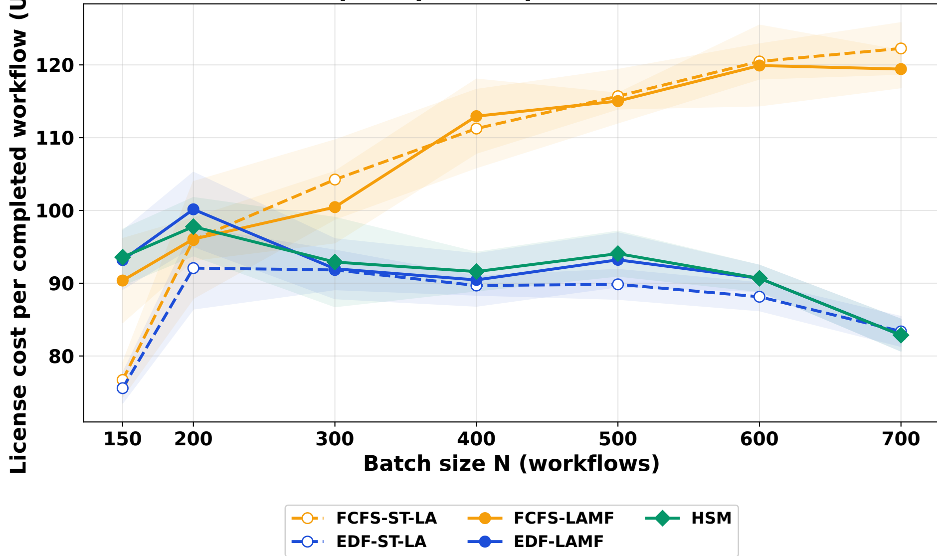
License spend per completed workflow vs N
