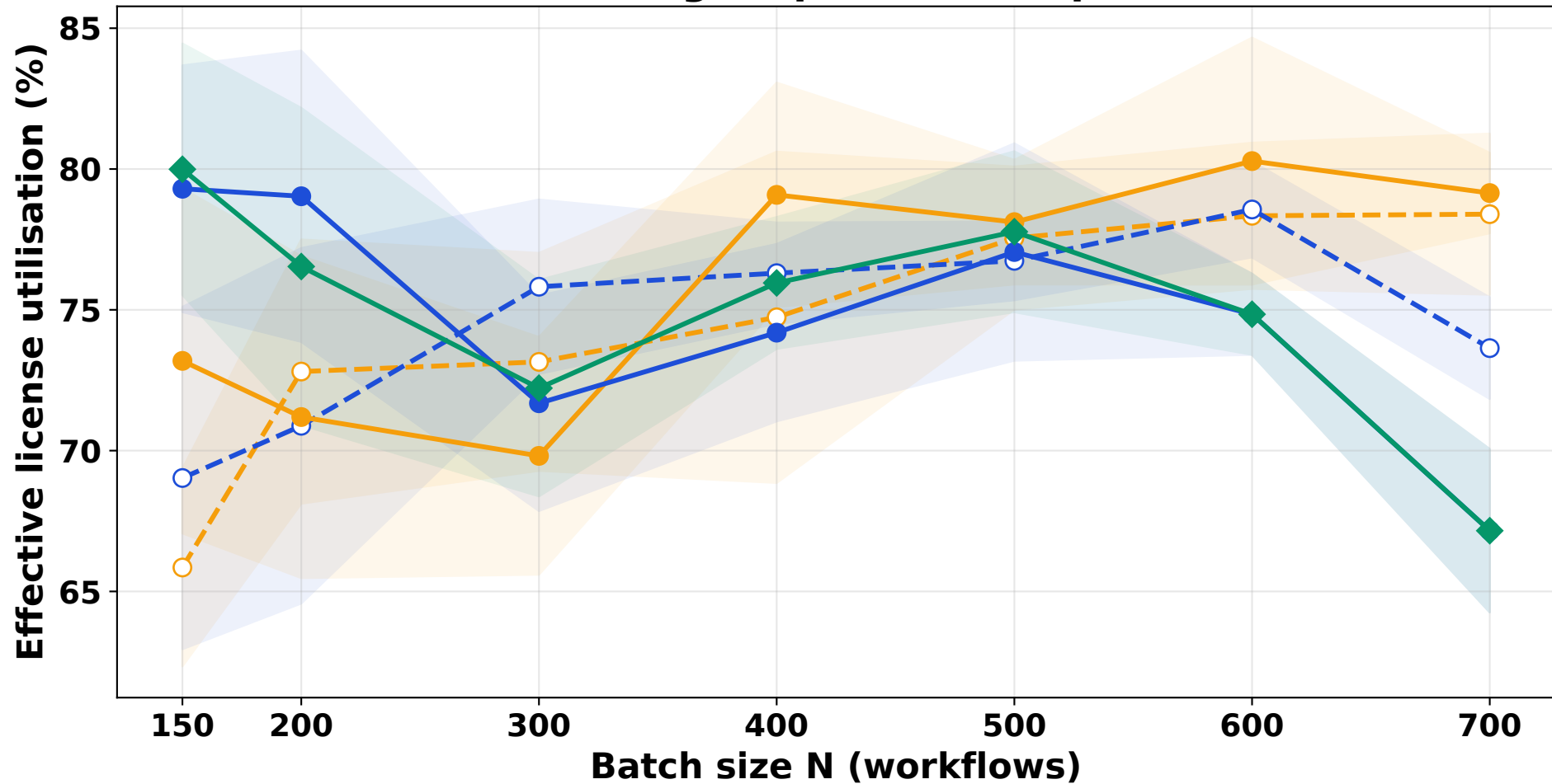
Share of license budget spent on completed work vs N
