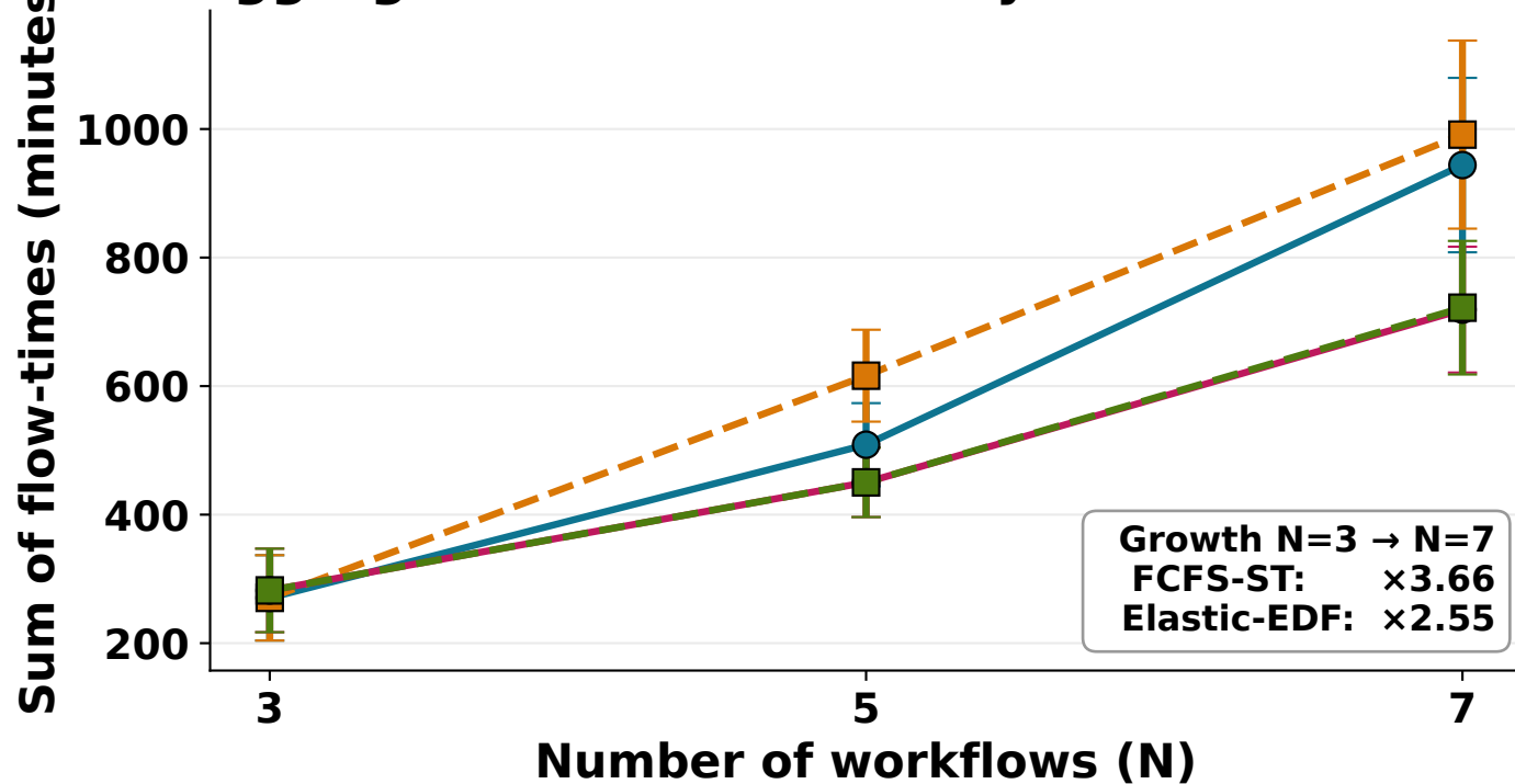
Aggregate workflow latency vs workload size
