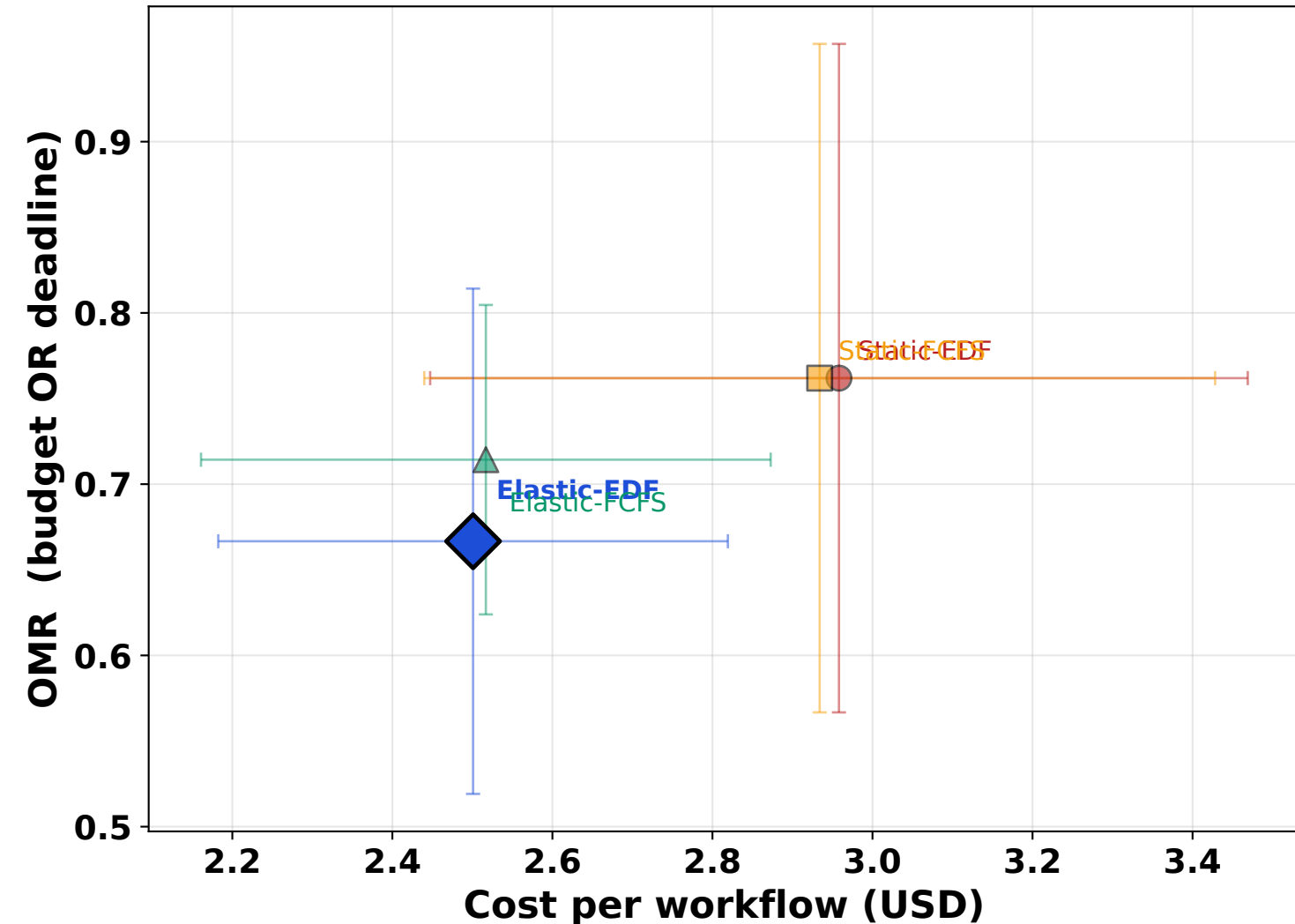
HPO @ N = 7
