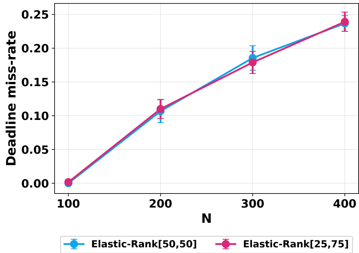
Deadline miss-rate vs N
