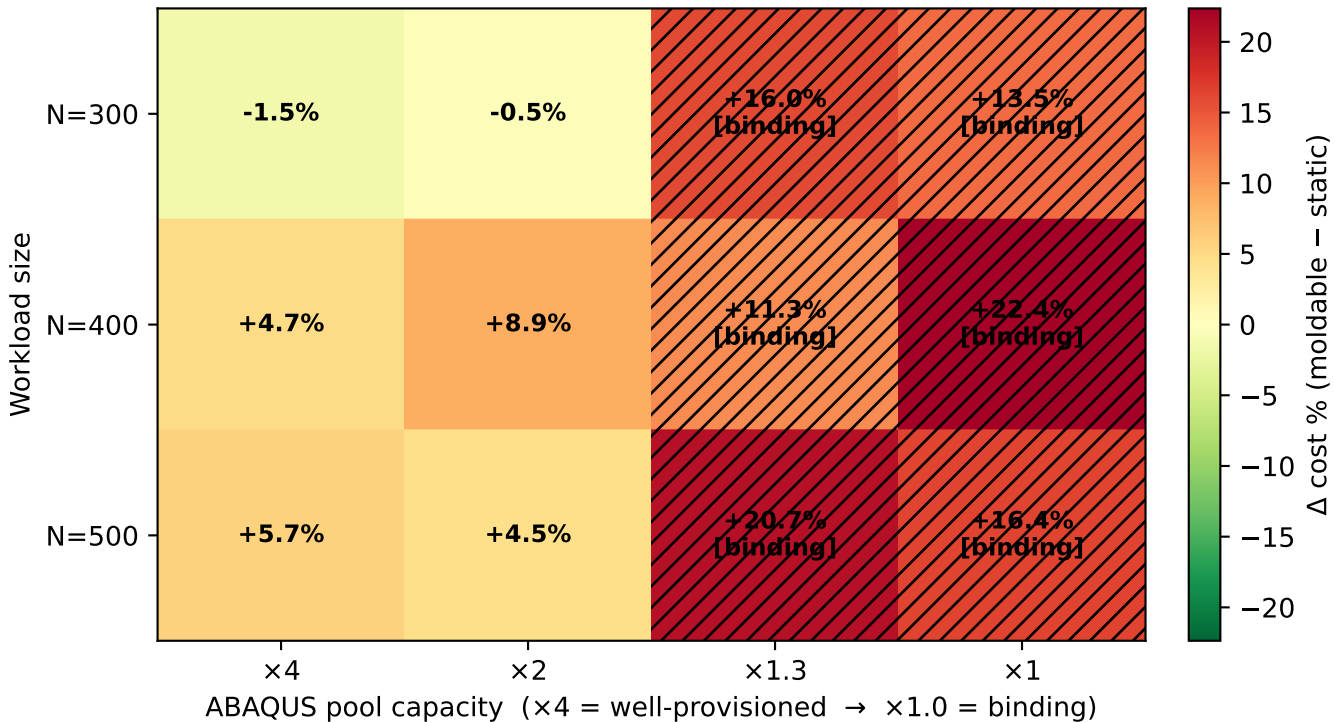
Moldable – Static EDF cost gap, 75% ABAQUS deck green = moldable parity/win, red = moldable worse
