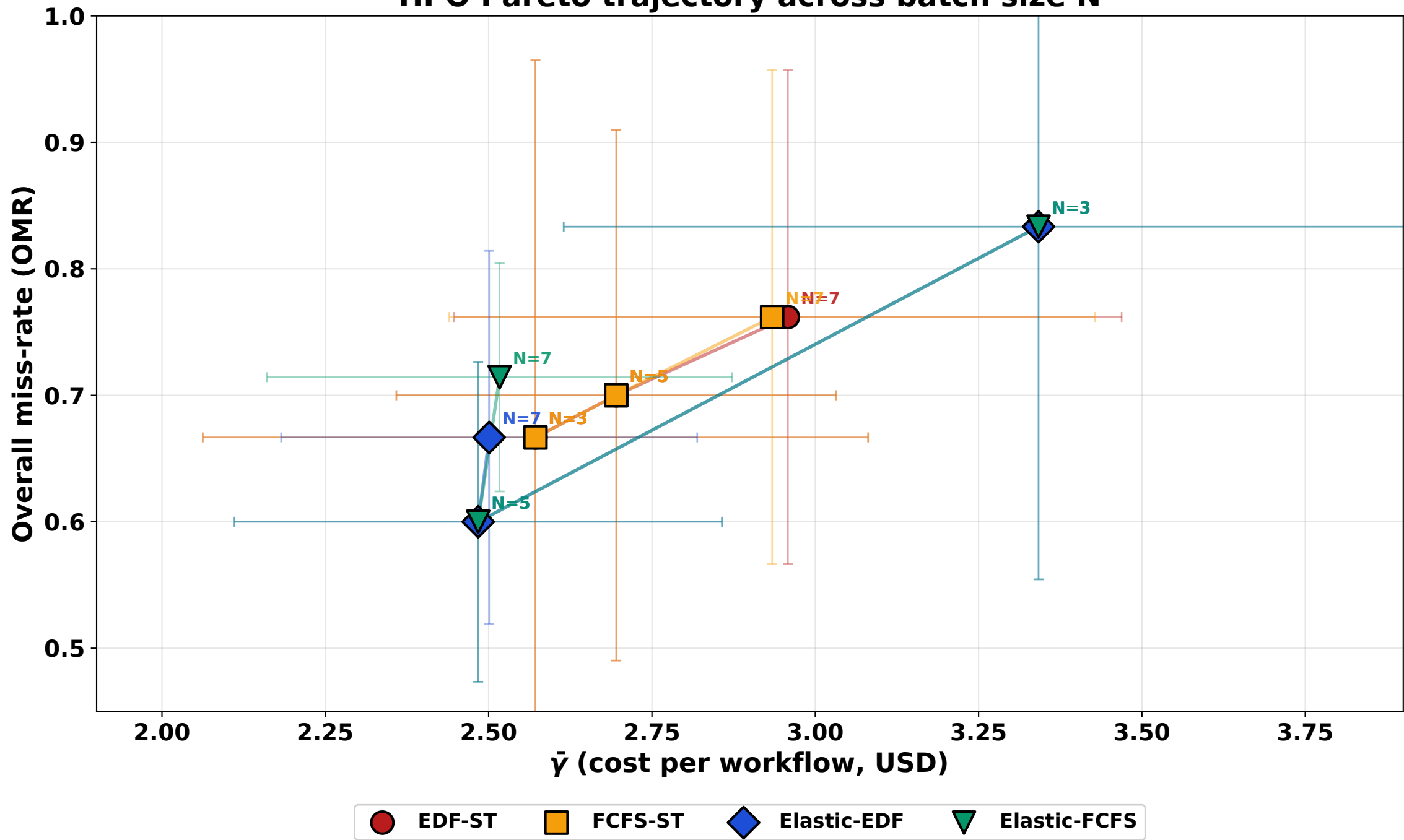
HPO Pareto trajectory across batch size N
