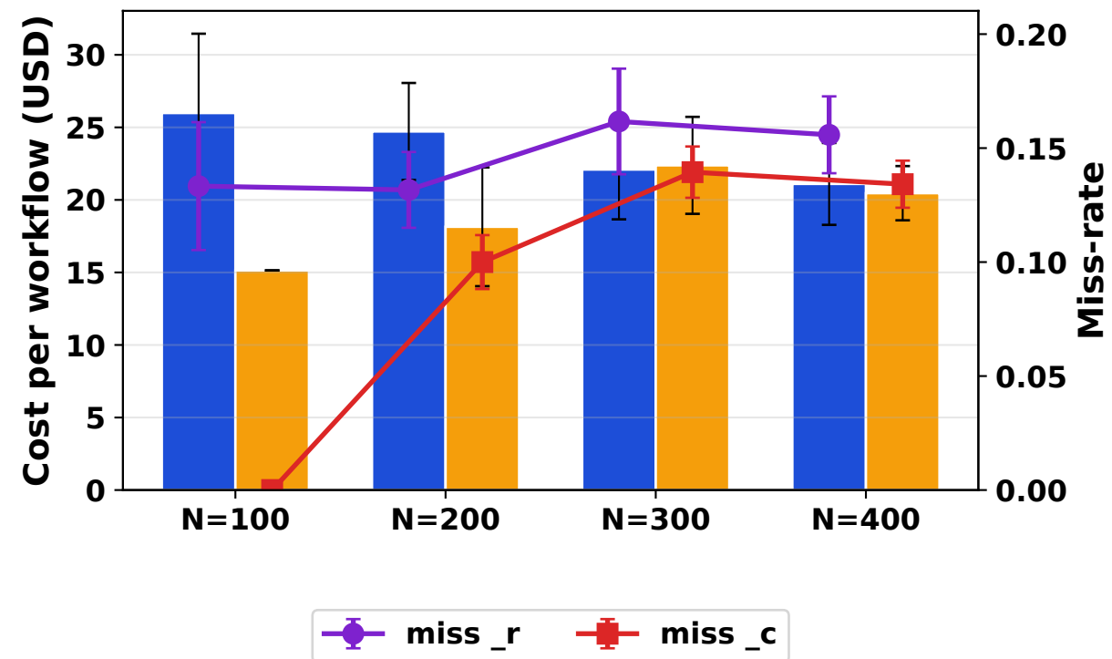
Elastic-EDF
