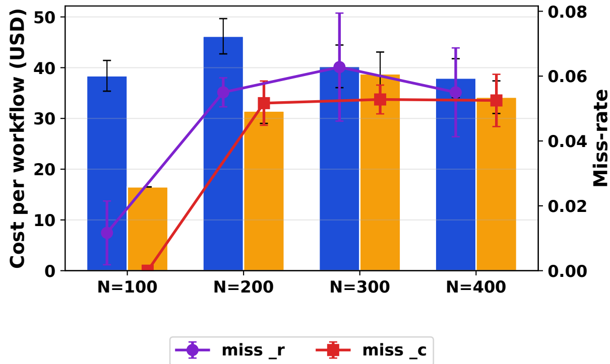
EDF-ST
