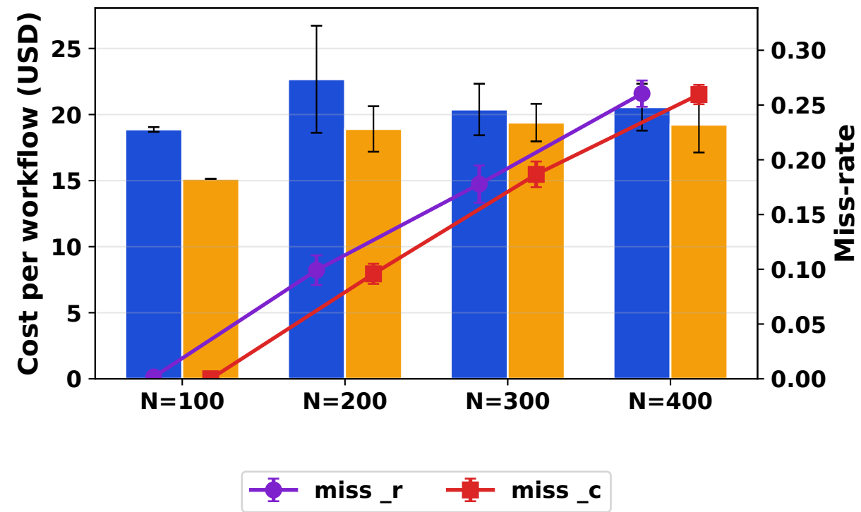
Elastic-FCFS
