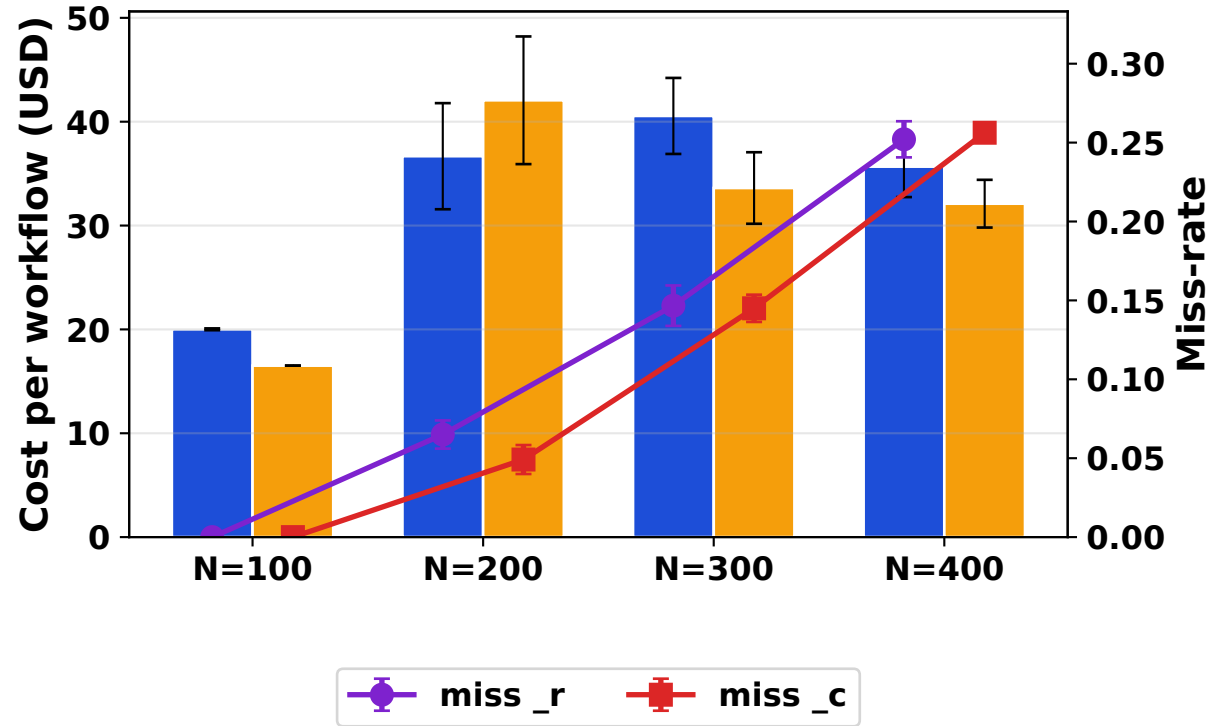
FCFS-ST
