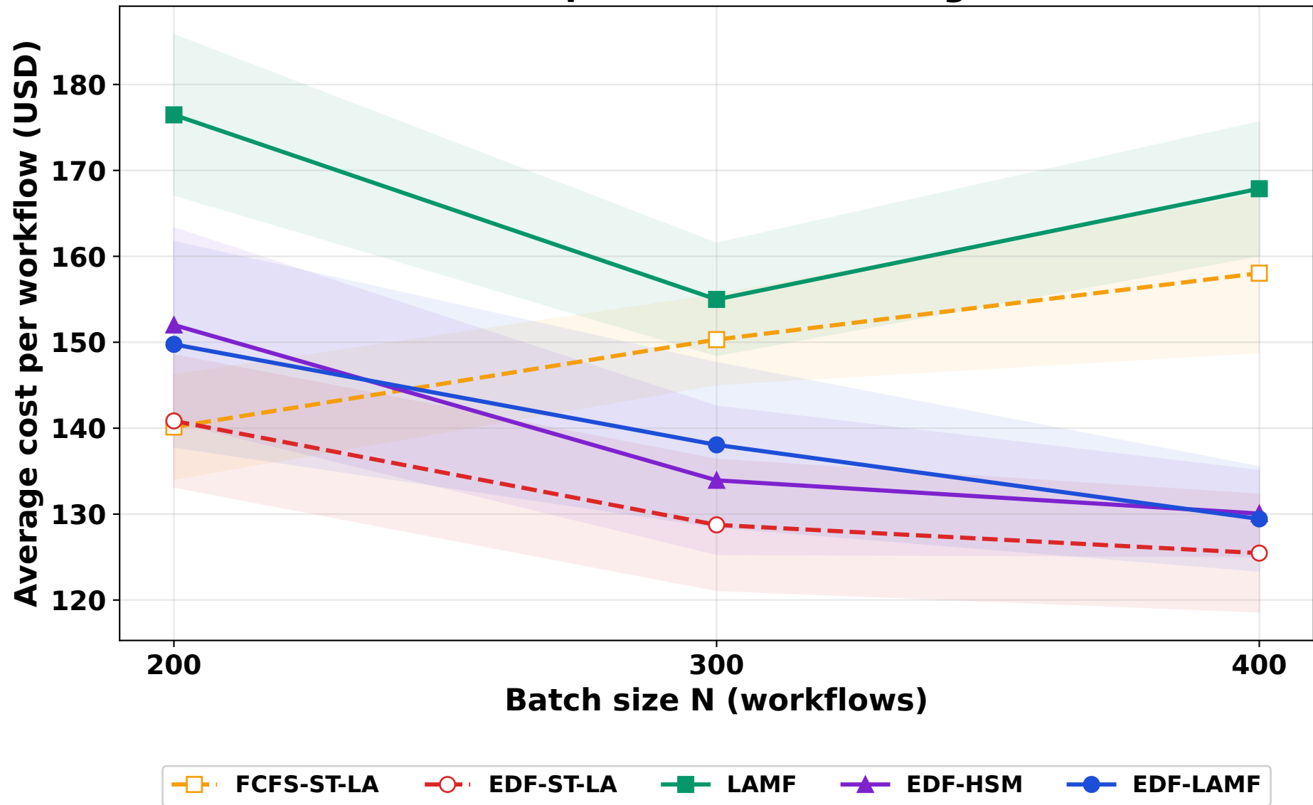
Cost-per-workflow scaling
