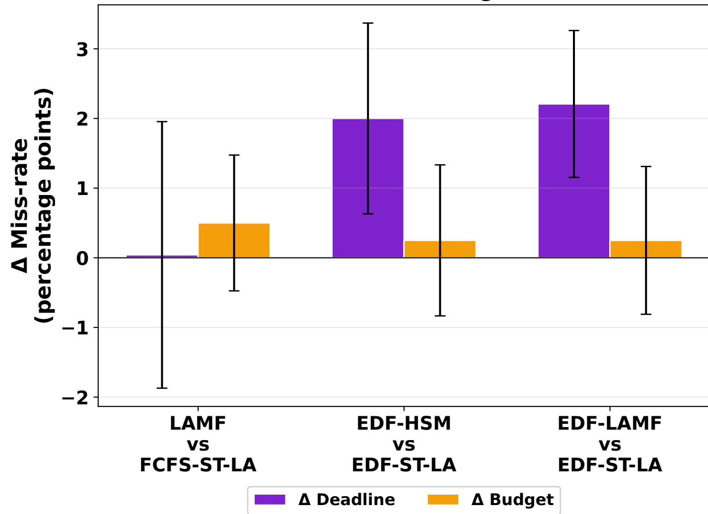
Miss-rate trade-off @ N=400
