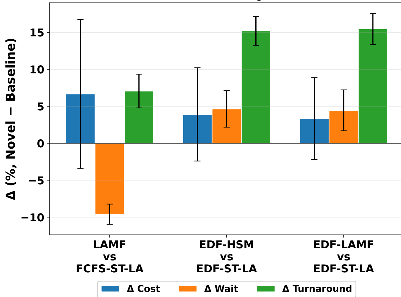
Relative deltas @ N=400
