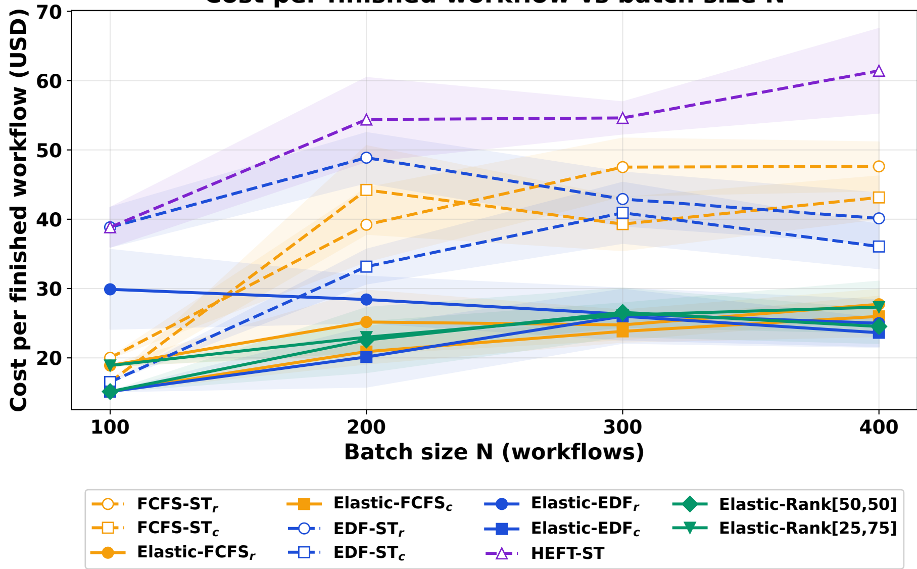
Cost per finished workflow vs batch size N
