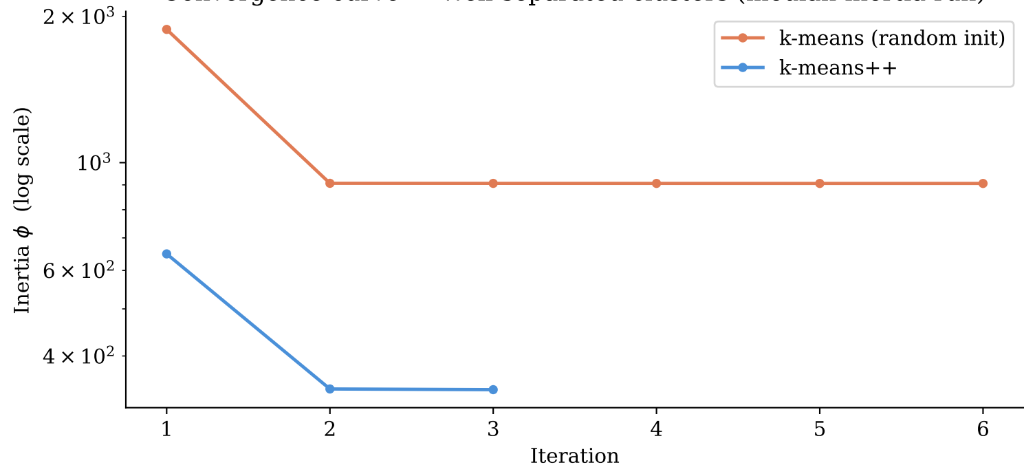
Convergence curve — Well-separated clusters (median-inertia run)
