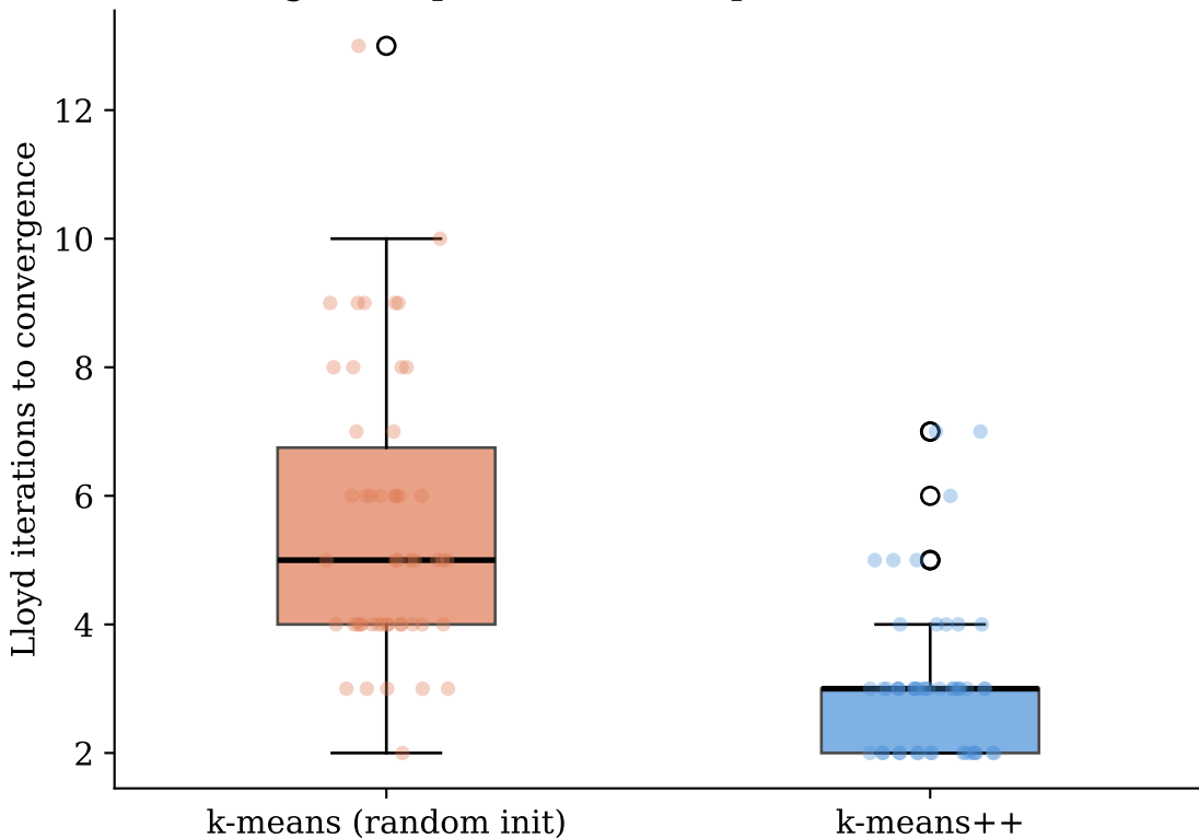
Convergence speed — Well-separated clusters (k=5)
