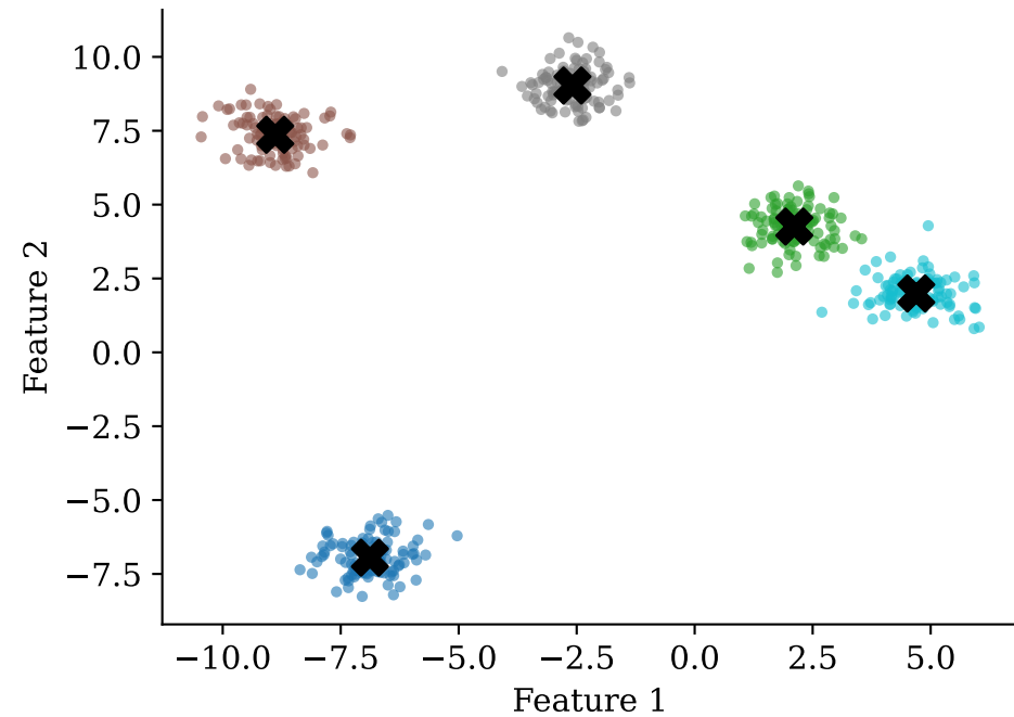
k-means++ — BEST run Inertia = 341
