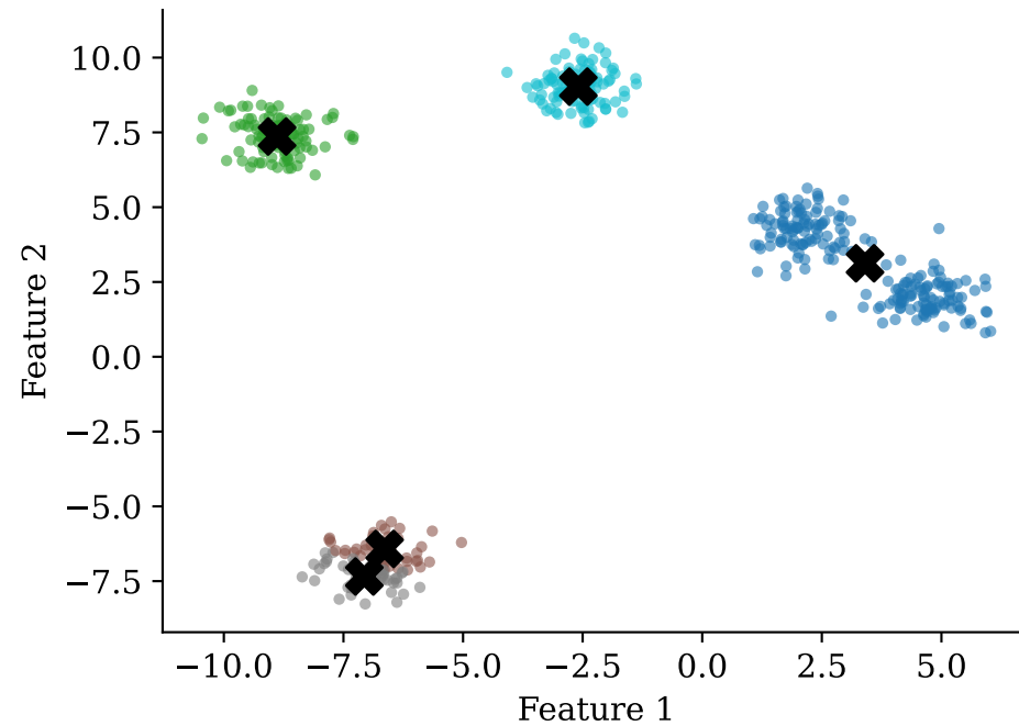
random init — typical (med) Inertia = 906
