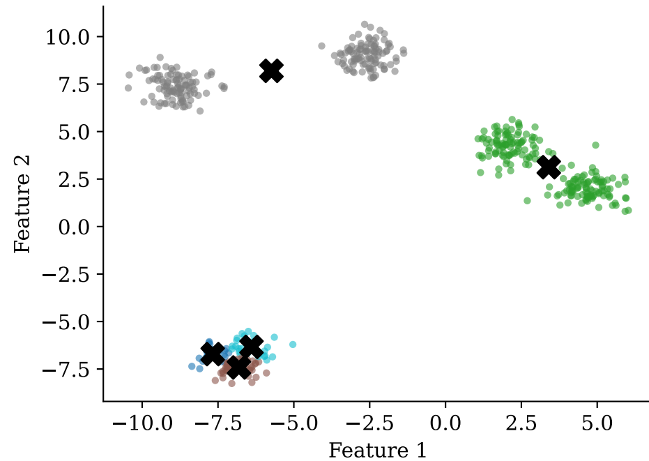
random init — WORST run Inertia = 3009
