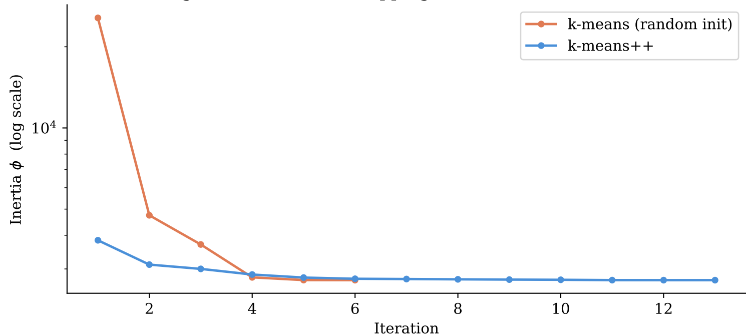
Convergence curve — Overlapping clusters (median-inertia run)
