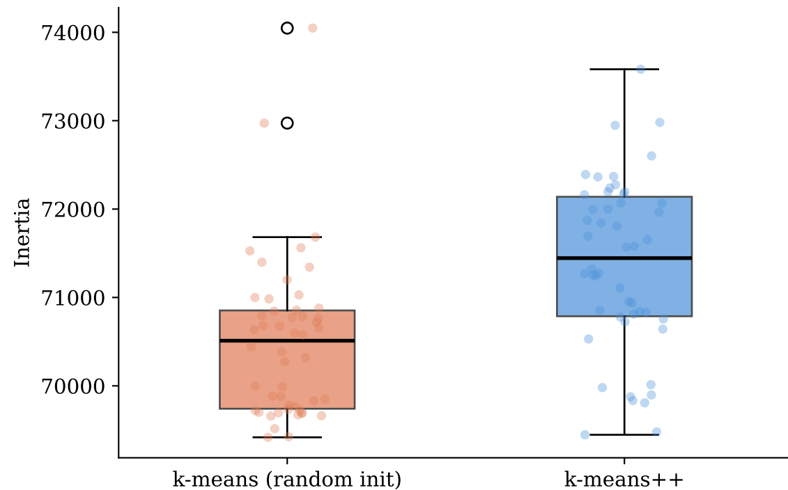
Inertia over 50 restarts
