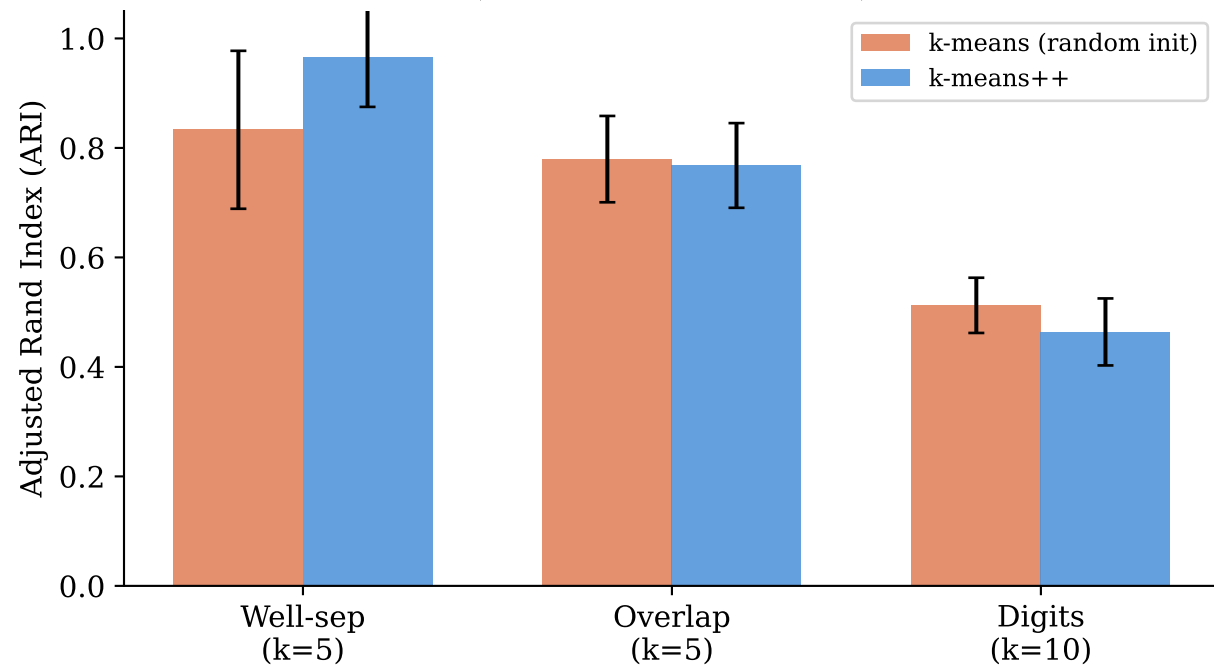
Adjusted Rand Index (ARI) vs ground-truth labels (mean \pm std, 50 trials)
