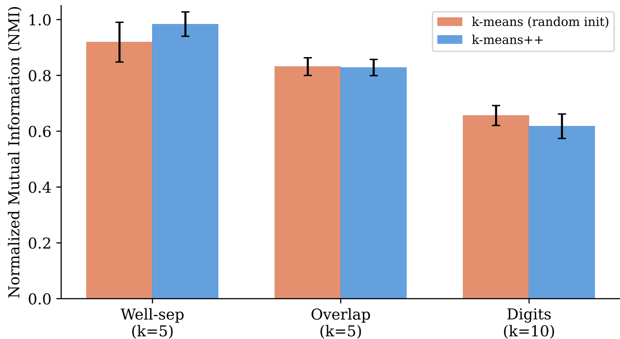
Normalized Mutual Information (NMI) vs ground-truth labels (mean \pm std, 50 trials)
