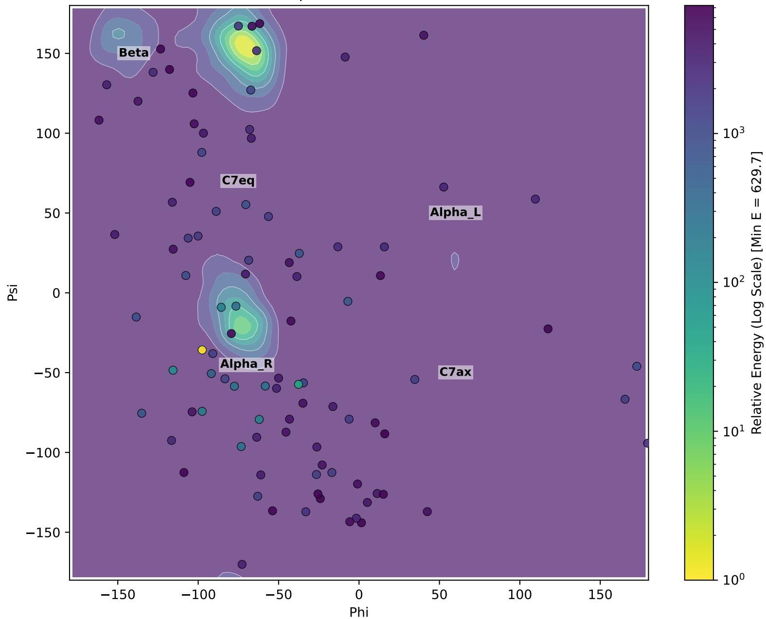
Refined Structures Colored by Log Relative Energy (Loop 23, 95 structures)
