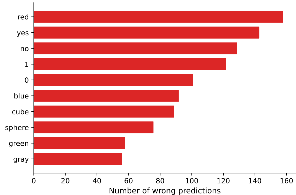
CoT: Most Common Wrong Predictions
