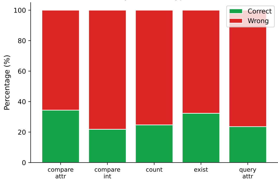
CoT: Correct vs. Wrong by Question Type
