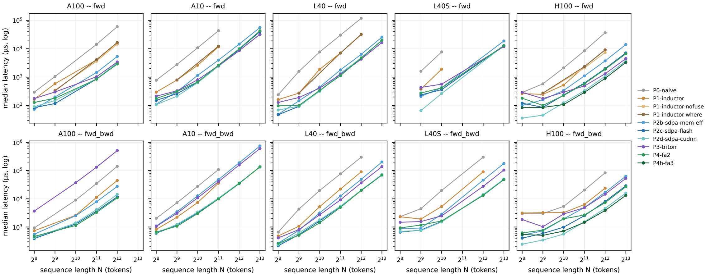
Prefix latency vs sequence length (causal, B=4, D=128, dt=bf16) log-log; each row of panels has its own y axis -- fwd and fwd_bwd are different measurements
