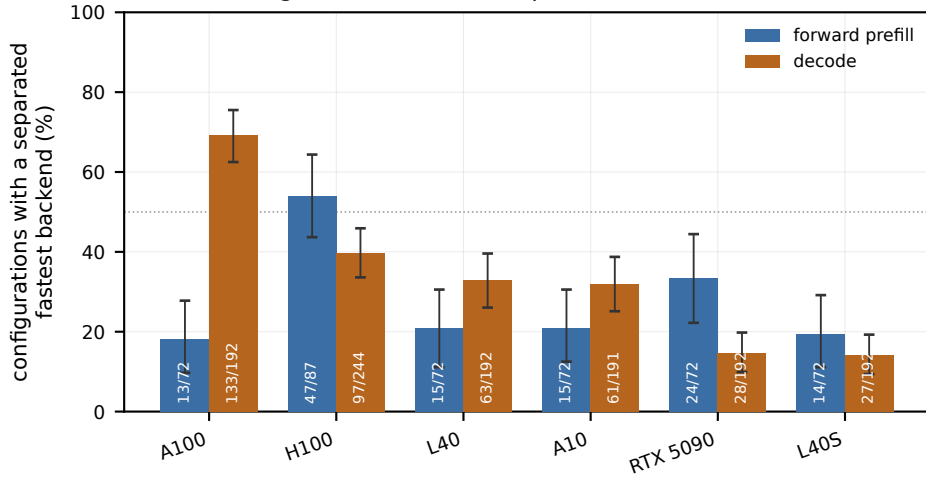
A Most configurations have no separated winner
