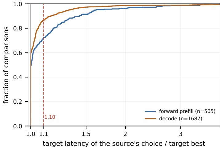
B Cost of transferring the choice prefill 14% unavailable on target; decode 15% unavailable on target
