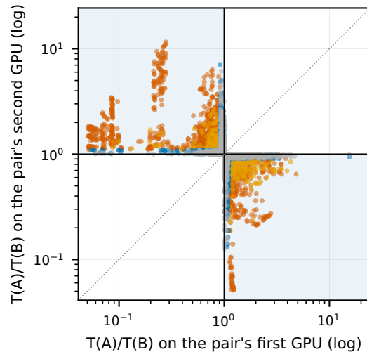
decode -- cross-architecture pairs (14 GPU pairs) 5142 sign flips, 682 past 10% both ways (2.9% of 23250 comparable pairs)
