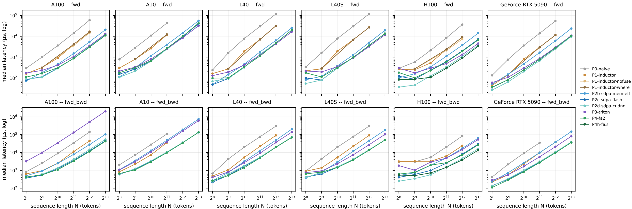
Prefill latency vs sequence length (causal, B=4, D=128, dt=bf16) log-log; each row of panels has its own y axis -- fwd and fwd_bwd are different measurements
