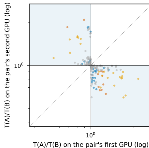
decode -- same-architecture control: L40 vs L40S 190 sign flips, 45 past 10% both ways (2.3% of 1950 comparable pairs)
