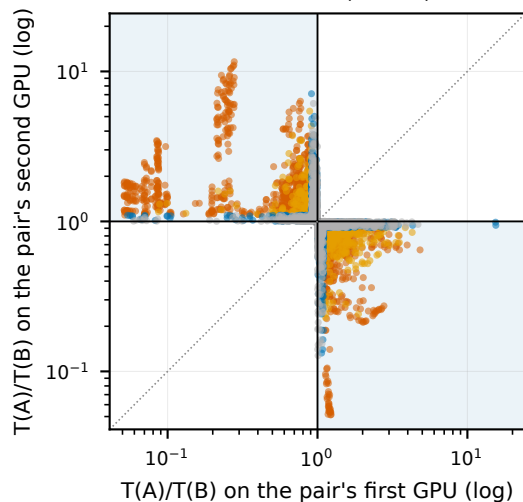
decode -- cross-architecture pairs (14 GPU pairs) 5119 sign flips, 674 past 10% both ways (2.9% of 22905 comparable pairs)
