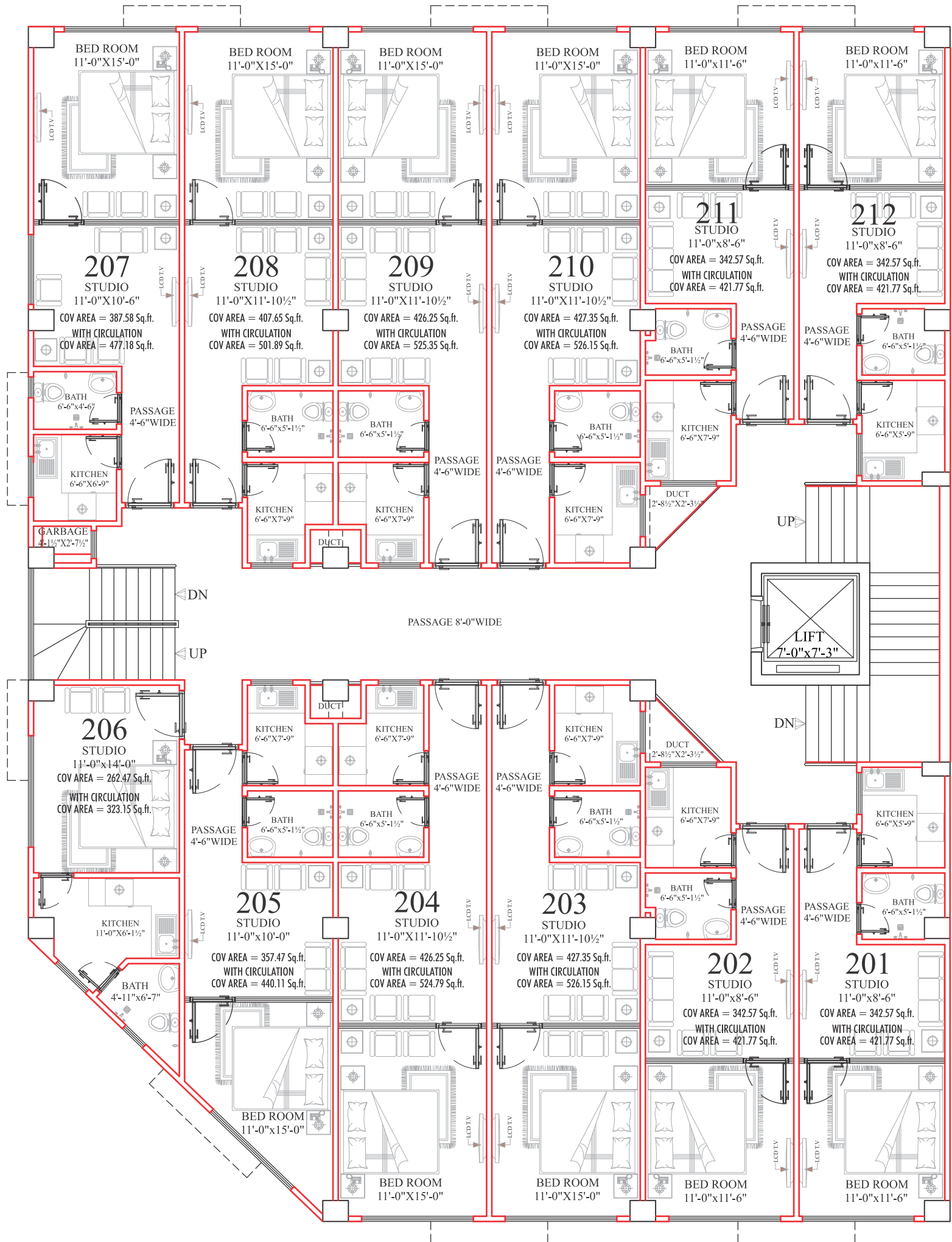
2nd FLOOR LAYOUT PLAN COV AREA = 5429.53 Sq.ft. CIR AREA = 907.48 Sq.ft. NOTE:- ALL TEXT INCLUDING WALL
