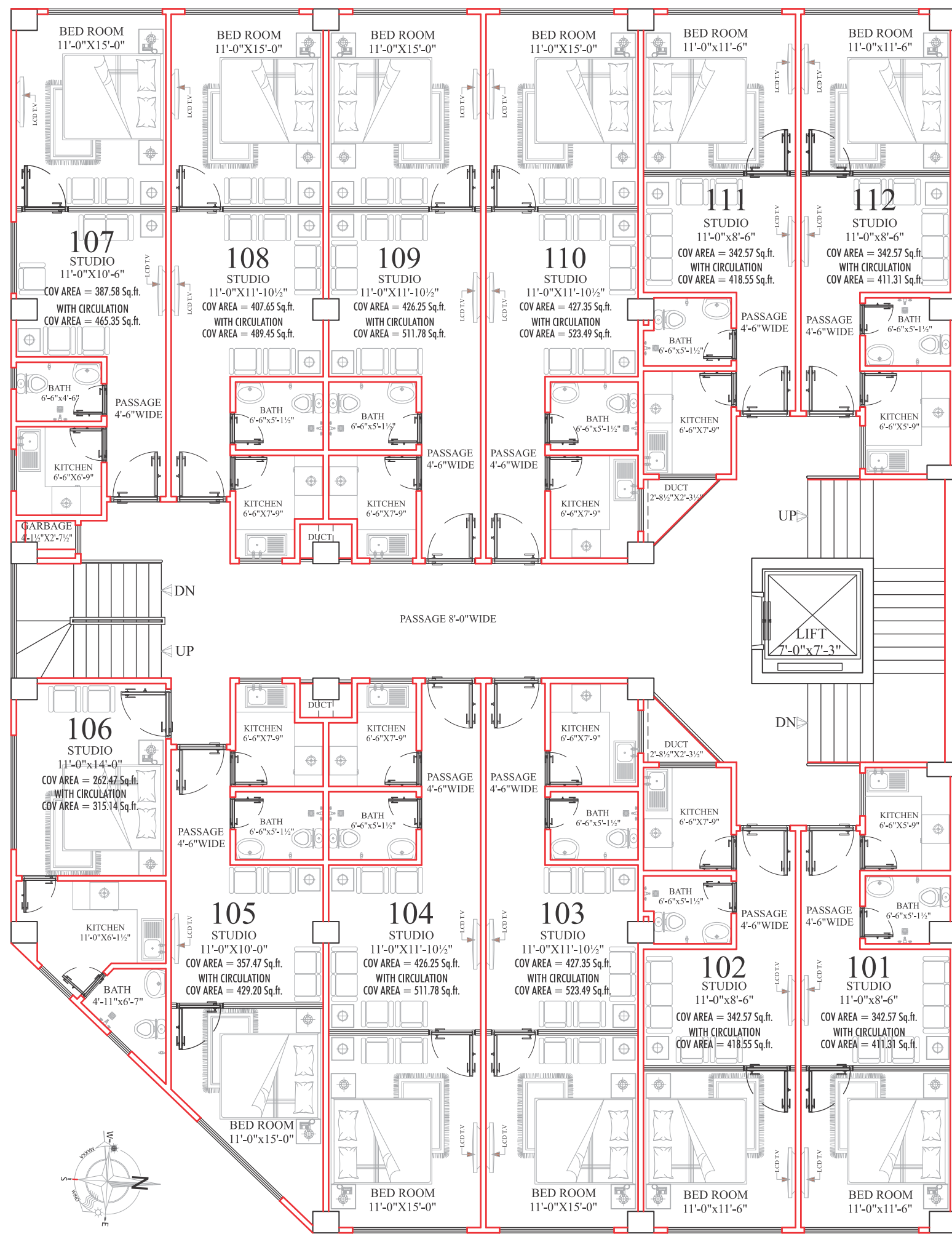
FIRST FLOOR LAYOUT PLAN COV AREA = 5429.53 Sq.ft. CIR AREA = 907.48 Sq.ft. NOTE:- ALL TEXT INCLUDING WALL
