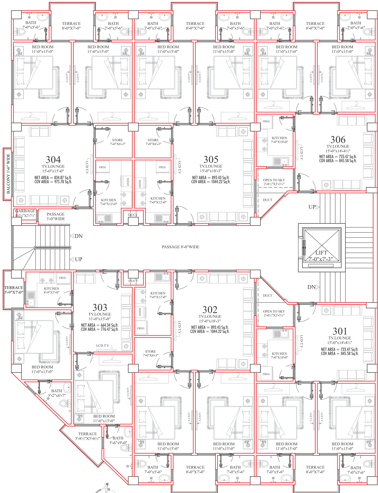
3rd FLOOR LAYOUT PLAN COV AREA = 5531.90 Sq.ft. CIR AREA = 798.87 Sq.ft. NOTE:- ALL TEXT INCLUDING WALL
