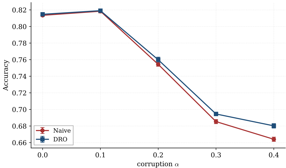
Adult Accuracy vs \alpha — COMBINED attack ( \tau=1 )
