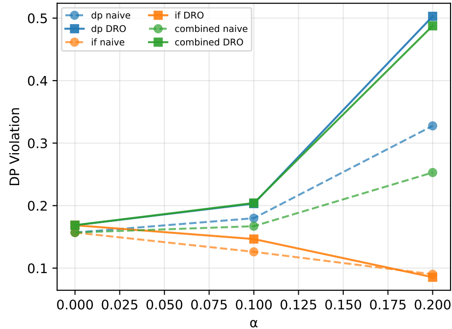
ADULT
