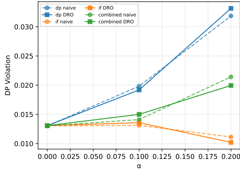
CREDIT
