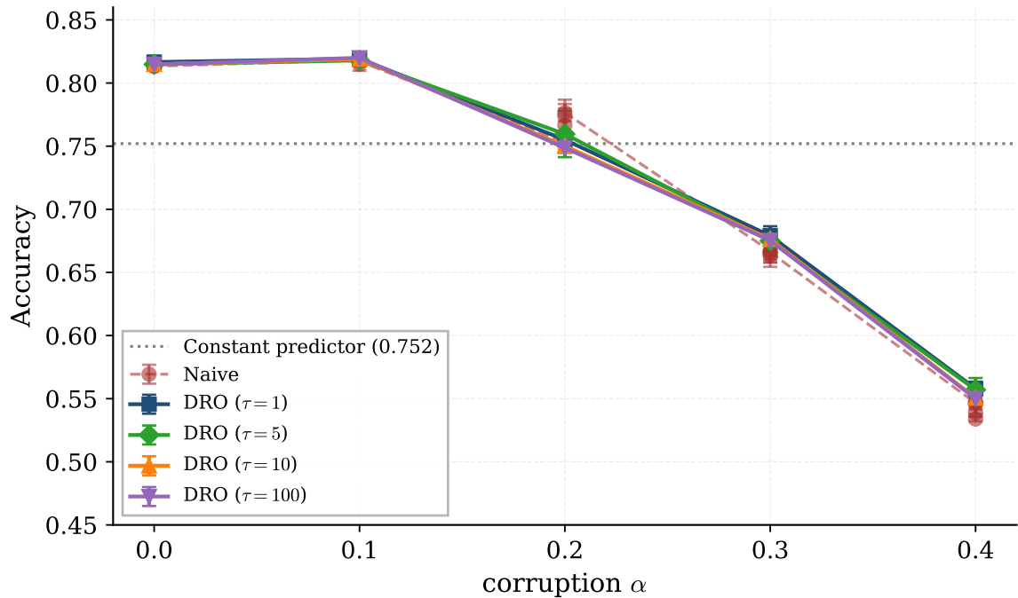
Accuracy vs \alpha — Adult (attack=DP)
