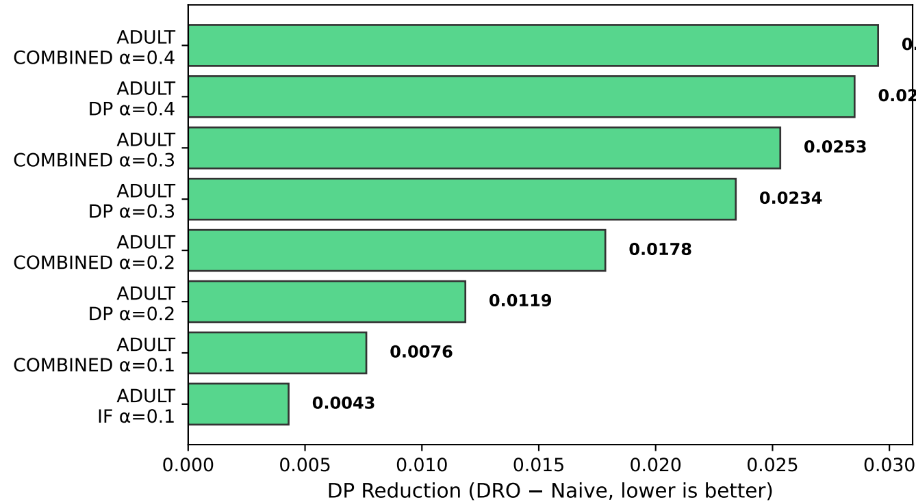
DRO vs Naive: Statistically Significant DP Wins (Wilcoxon p < 0.05 , n=6 seeds, \tau=1 fixed)
