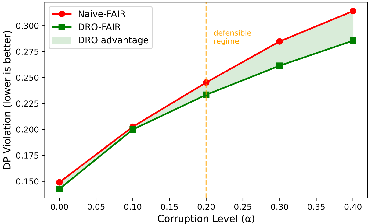
Adult — DP Attack: DRO vs Naive ( \tau=1 fixed, K_{\text{inner}}=10 , 6 seeds)
