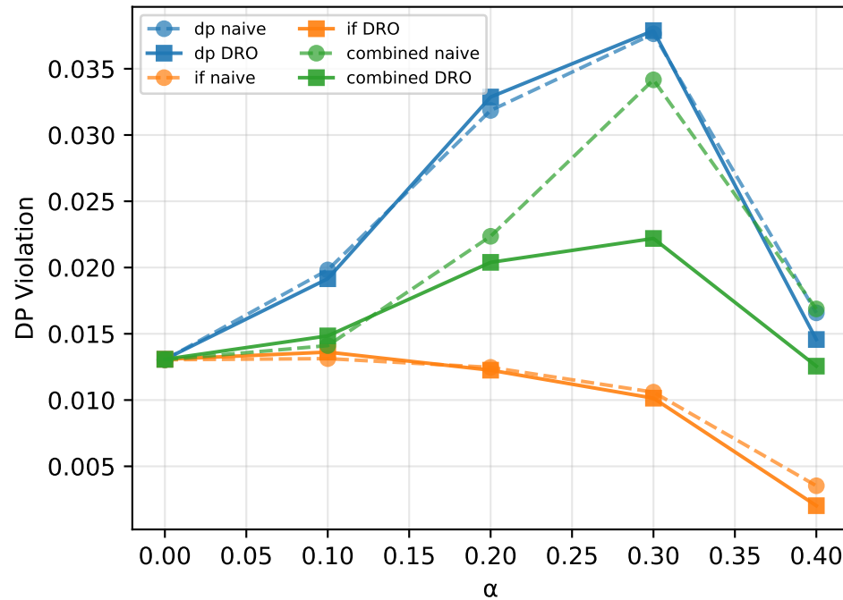
CREDIT
