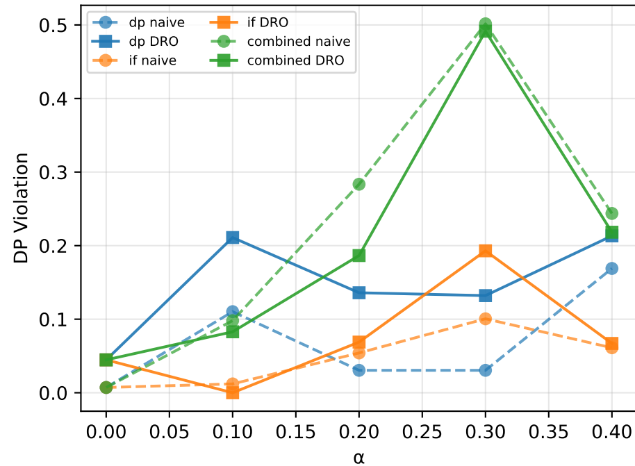
LSAC
