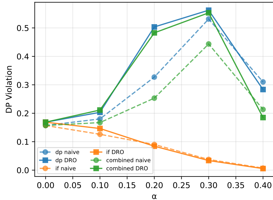
ADULT
