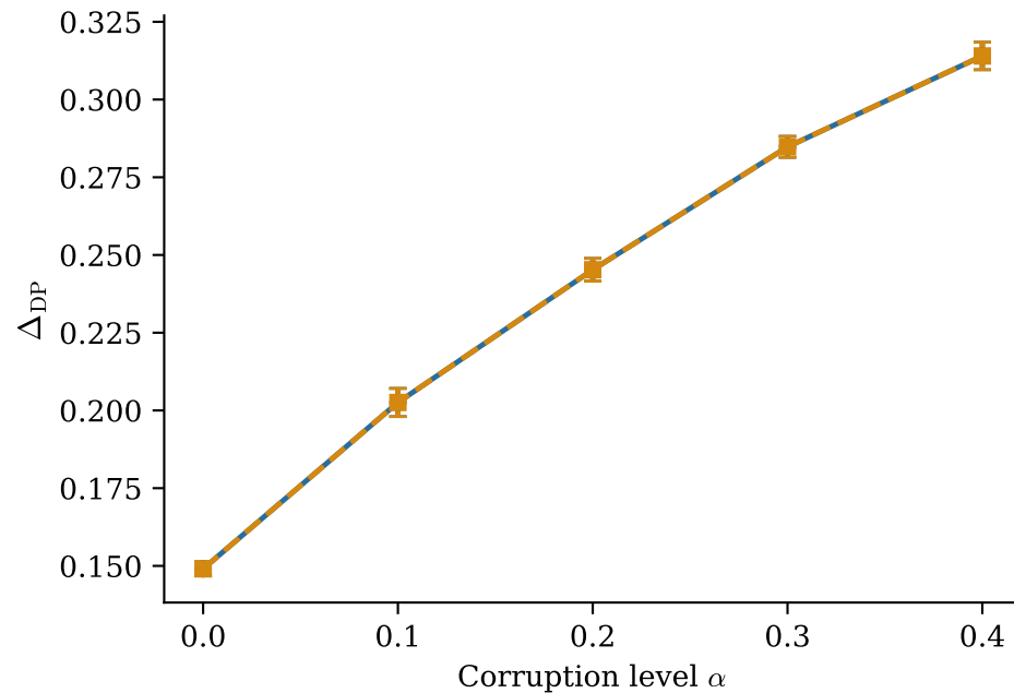
Adult — Naive-FAIR
