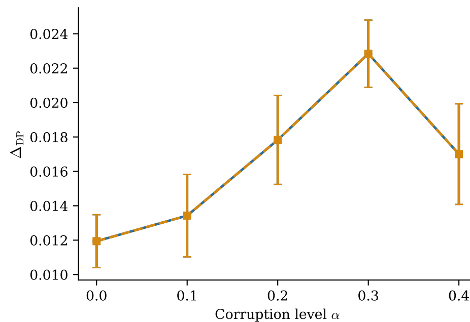
Credit — DRO-FAIR
