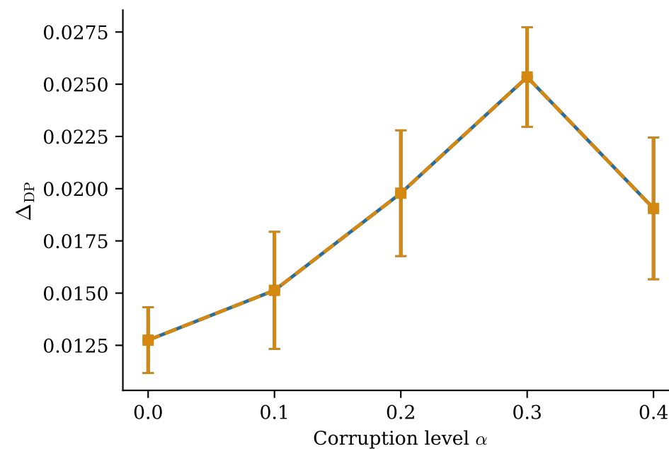
Credit — Naive-FAIR
