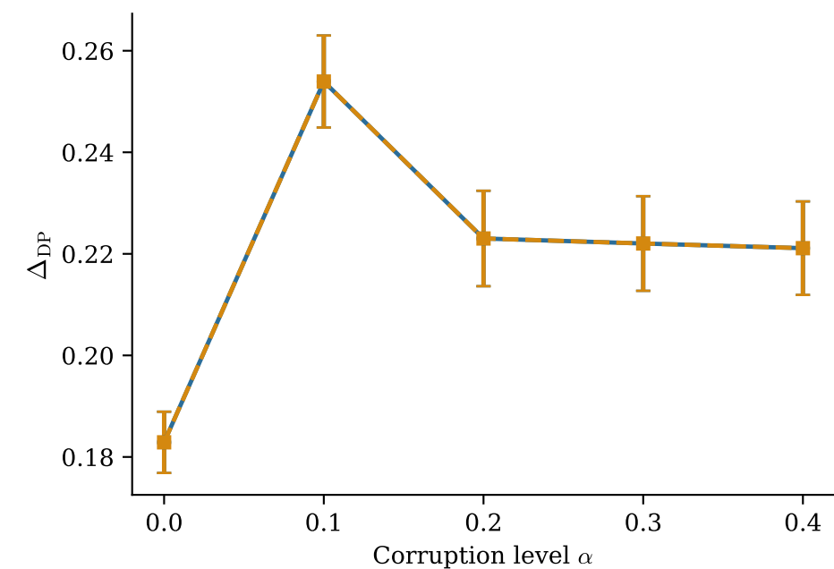
LSAC — DRO-FAIR
