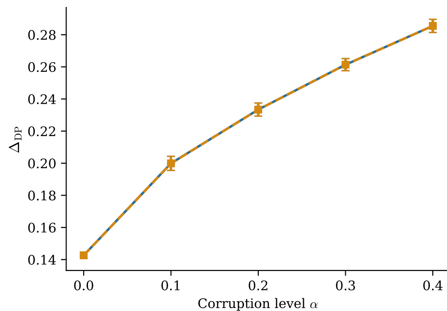
Adult — DRO-FAIR
