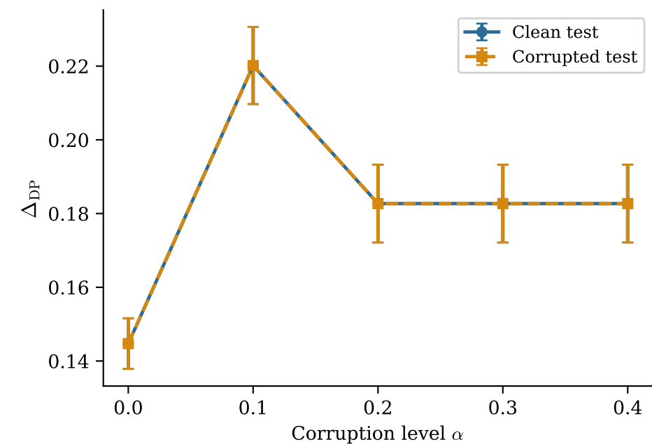
LSAC — Naive-FAIR
