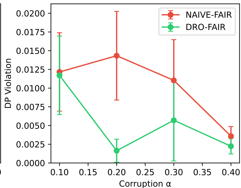
LSAC — IF-Attack
