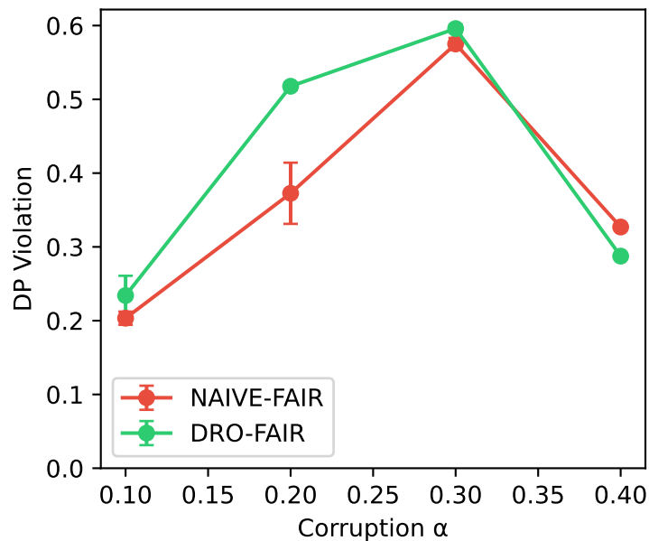
CREDIT — DP-Attack
