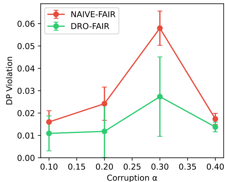
LSAC — COMBINED-Attack
