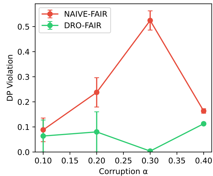
LSAC — COMBINED-Attack
