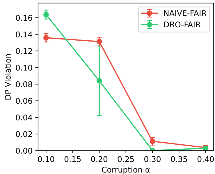
CREDIT — IF-Attack
