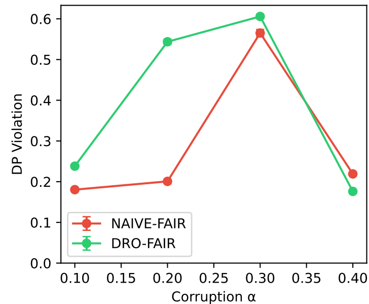
CREDIT — COMBINED-Attack
