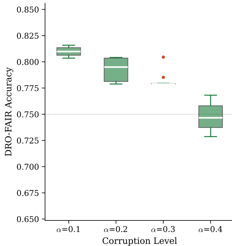
Credit
