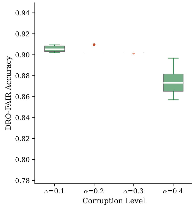
LSAC
