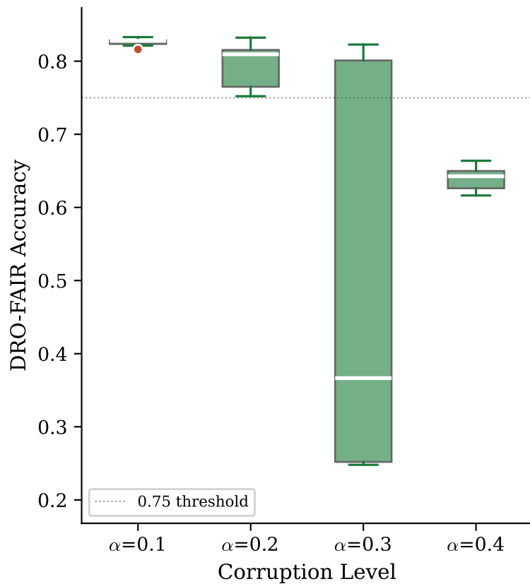
Adult
