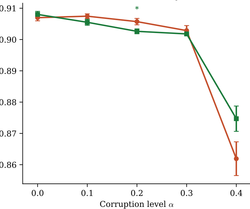
LSAC — Accuracy
