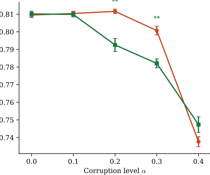
Credit — Accuracy
