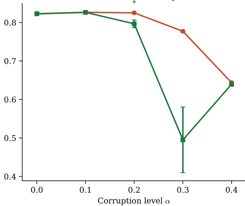
Adult — Accuracy
