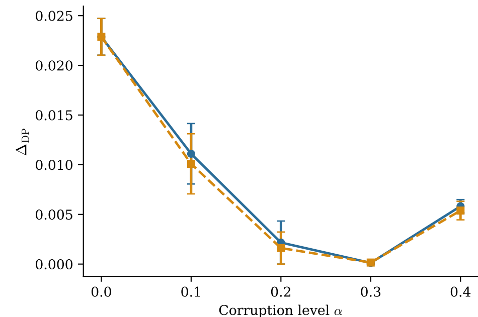
LSAC — DRO-FAIR
