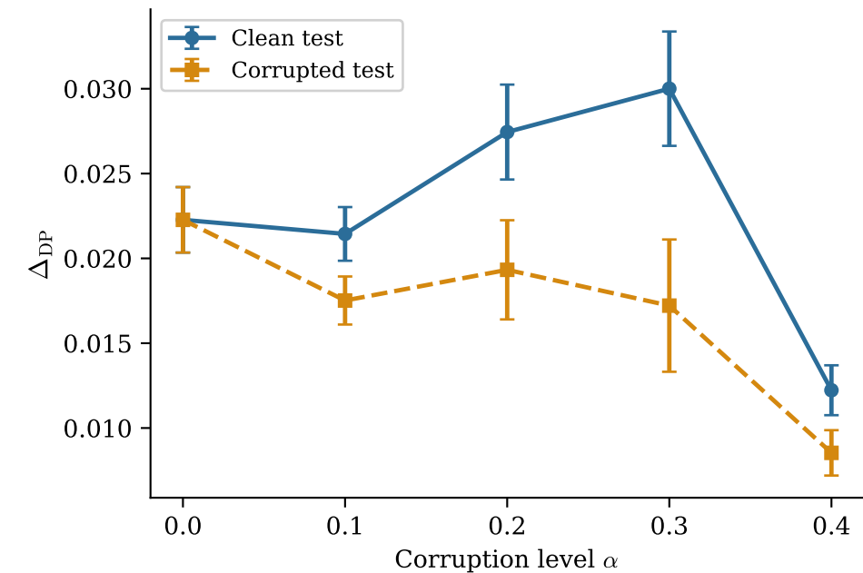
LSAC — Naive-FAIR
