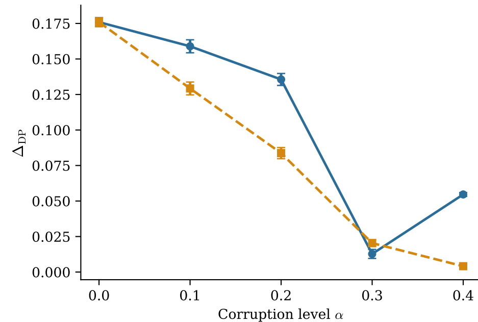
Adult — Naive-FAIR
