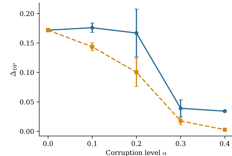
Adult — DRO-FAIR
