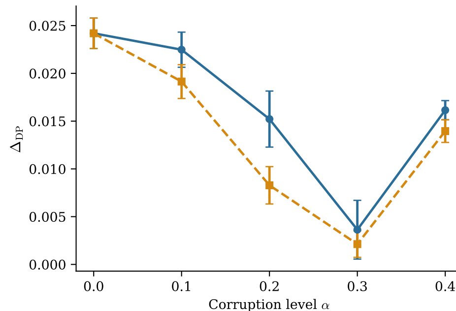
Credit — DRO-FAIR
