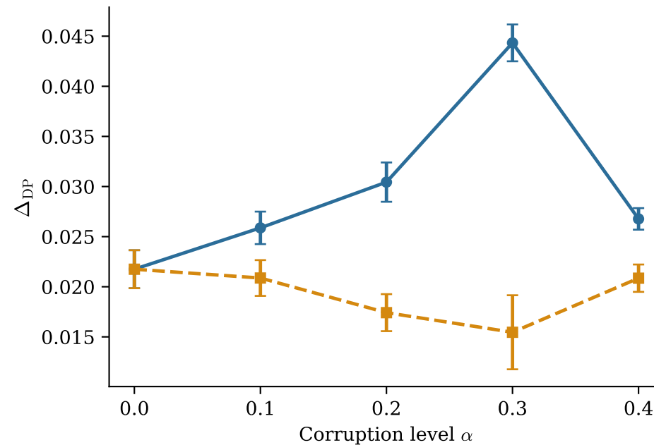
Credit — Naive-FAIR
