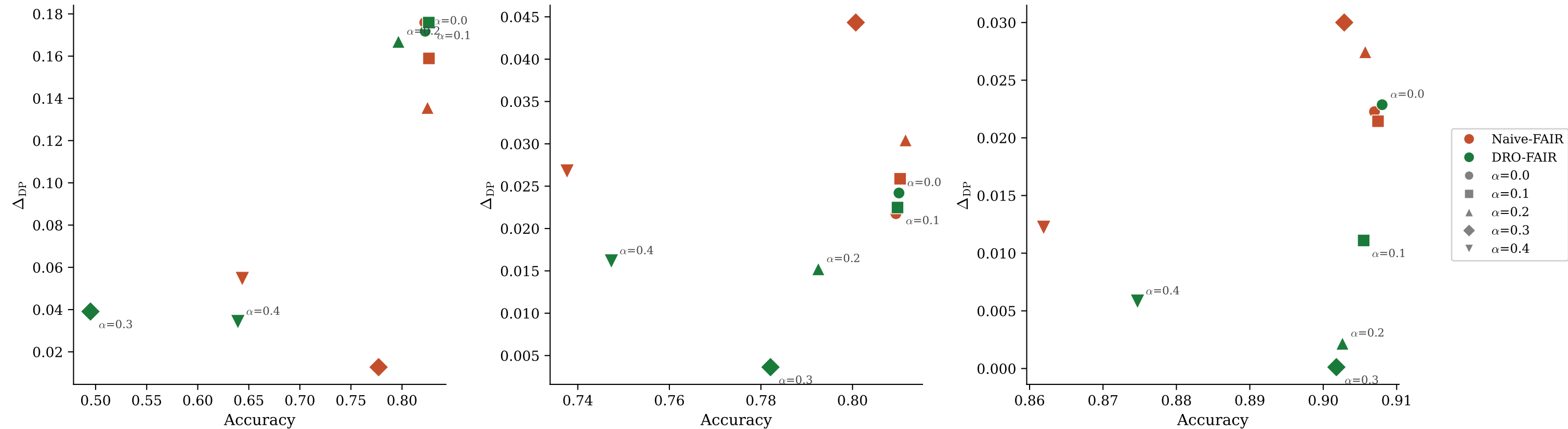
Accuracy vs Fairness Tradeoff (mean over 10 seeds, clean test)
