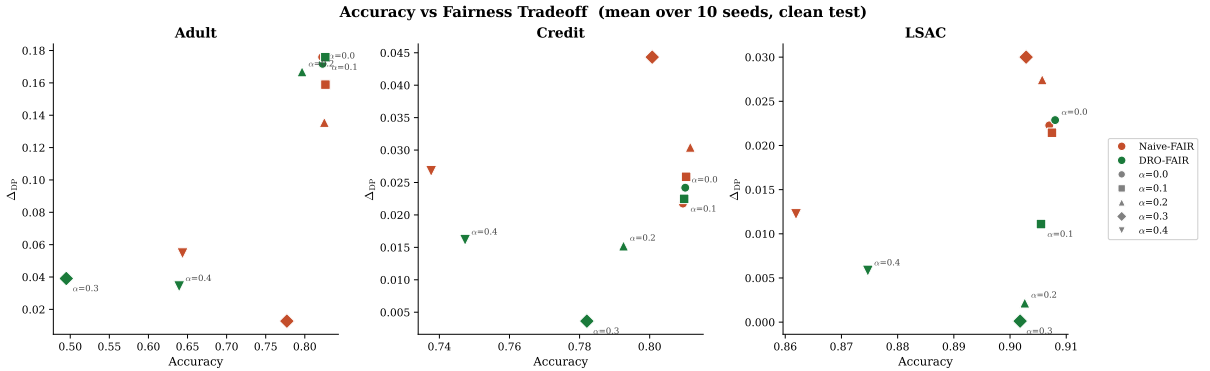
Figure 4: Accuracy-Fairness Tradeoff. Lower-right = high accuracy + low DP (ideal). DRO-FAIR moves toward lower DP on Credit/LSAC with minimal accuracy loss. Adult \alpha = 0.3 (DRO) is a clear outlier.
